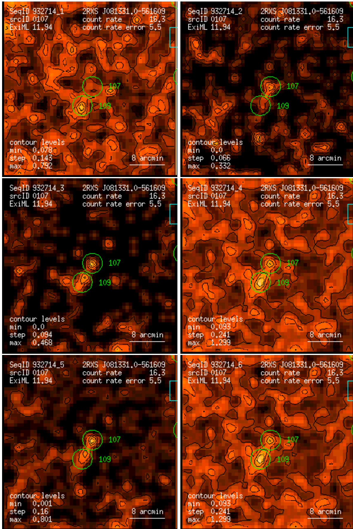
Figure 107: RASS 932714: detection 0107: band rate images, Gaussian filter: (1) PSPC channels 11 – 41, (2) 52 – 90, (3) 91 – 201, (4) 11 – 235, (5) 52 – 201, (6) 11 – 201. Broad band rates in counts/ks. Band rate contour levels in counts/ks/arcmin 2 .
