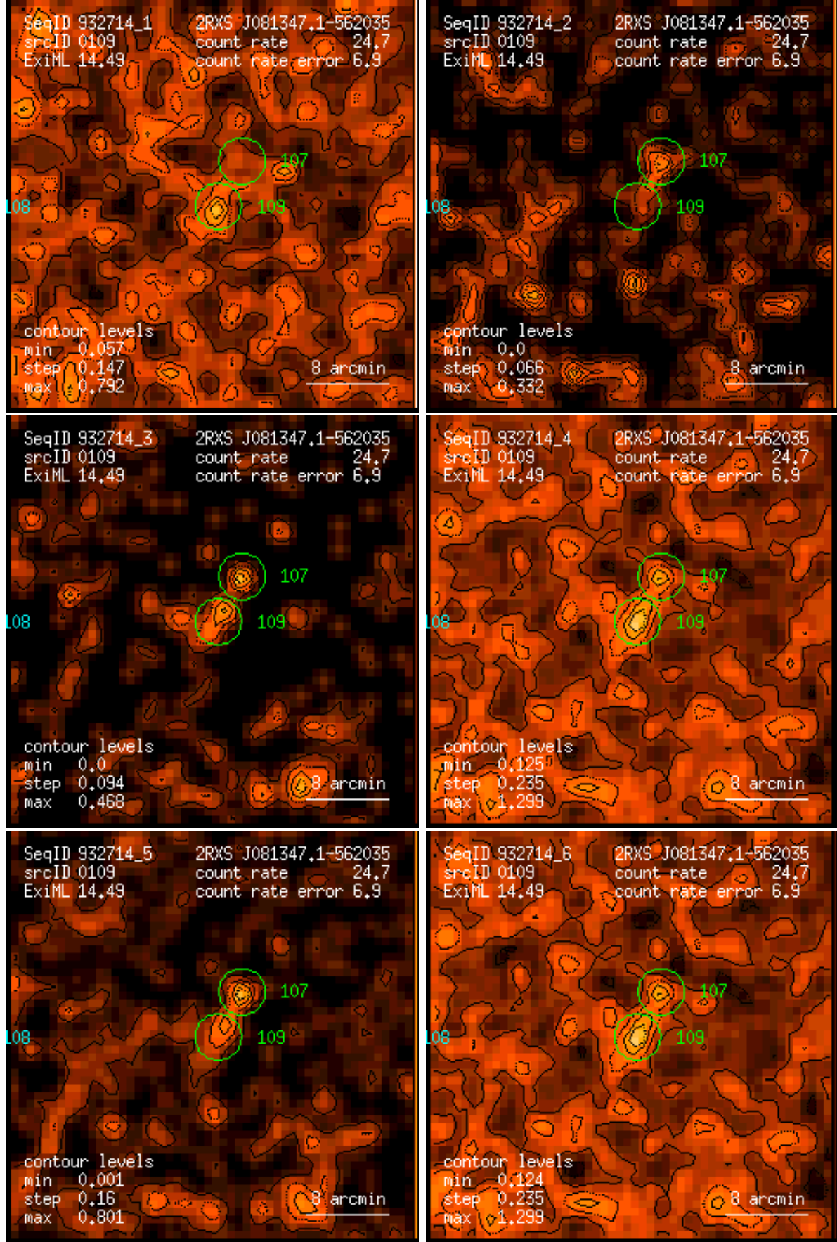
Figure 109: RASS 932714: detection 0109: band rate images, Gaussian filter: (1) PSPC channels 11 – 41, (2) 52 – 90, (3) 91 – 201, (4) 11 – 235, (5) 52 – 201, (6) 11 – 201. Broad band rates in counts/ks. Band rate contour levels in counts/ks/arcmin 2 .
