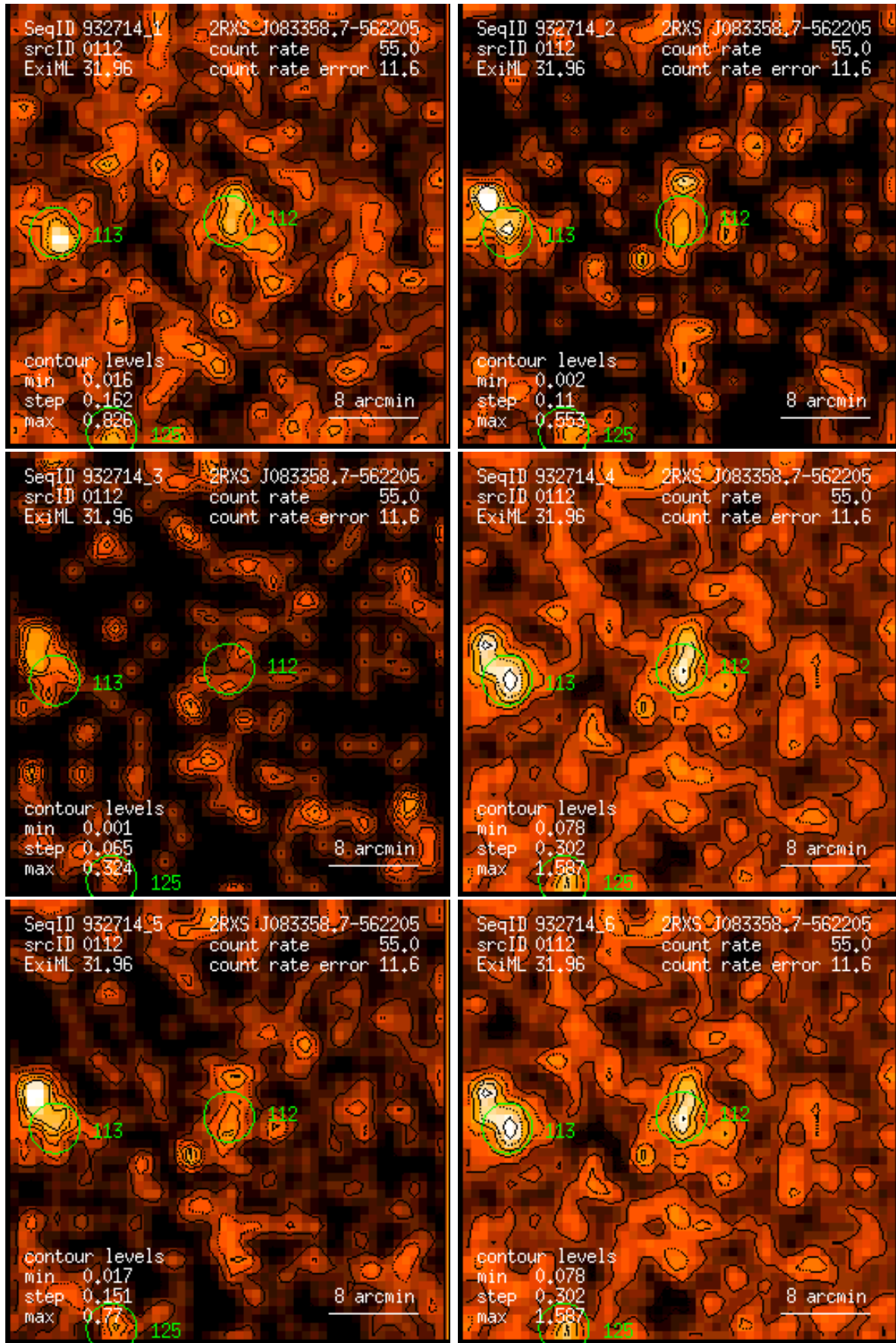
Figure 112: RASS 932714: detection 0112: band rate images, Gaussian filter: (1) PSPC channels 11 – 41, (2) 52 – 90, (3) 91 – 201, (4) 11 – 235, (5) 52 – 201, (6) 11 – 201. Broad band rates in counts/ks. Band rate contour levels in counts/ks/arcmin 2 .
