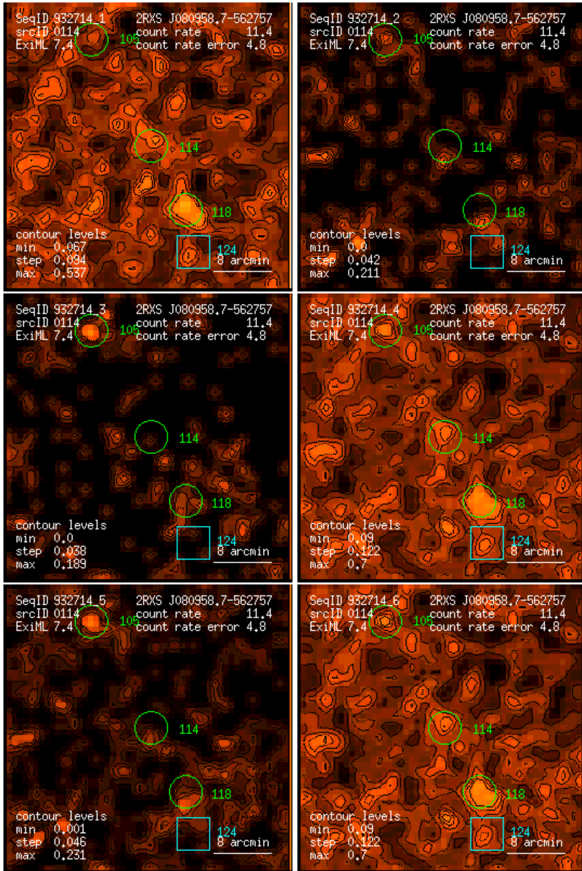
Figure 114: RASS 932714: detection 0114: band rate images, Gaussian filter: (1) PSPC channels 11 – 41, (2) 52 – 90, (3) 91 – 201, (4) 11 – 235, (5) 52 – 201, (6) 11 – 201. Broad band rates in counts/ks. Band rate contour levels in counts/ks/arcmin 2 .
