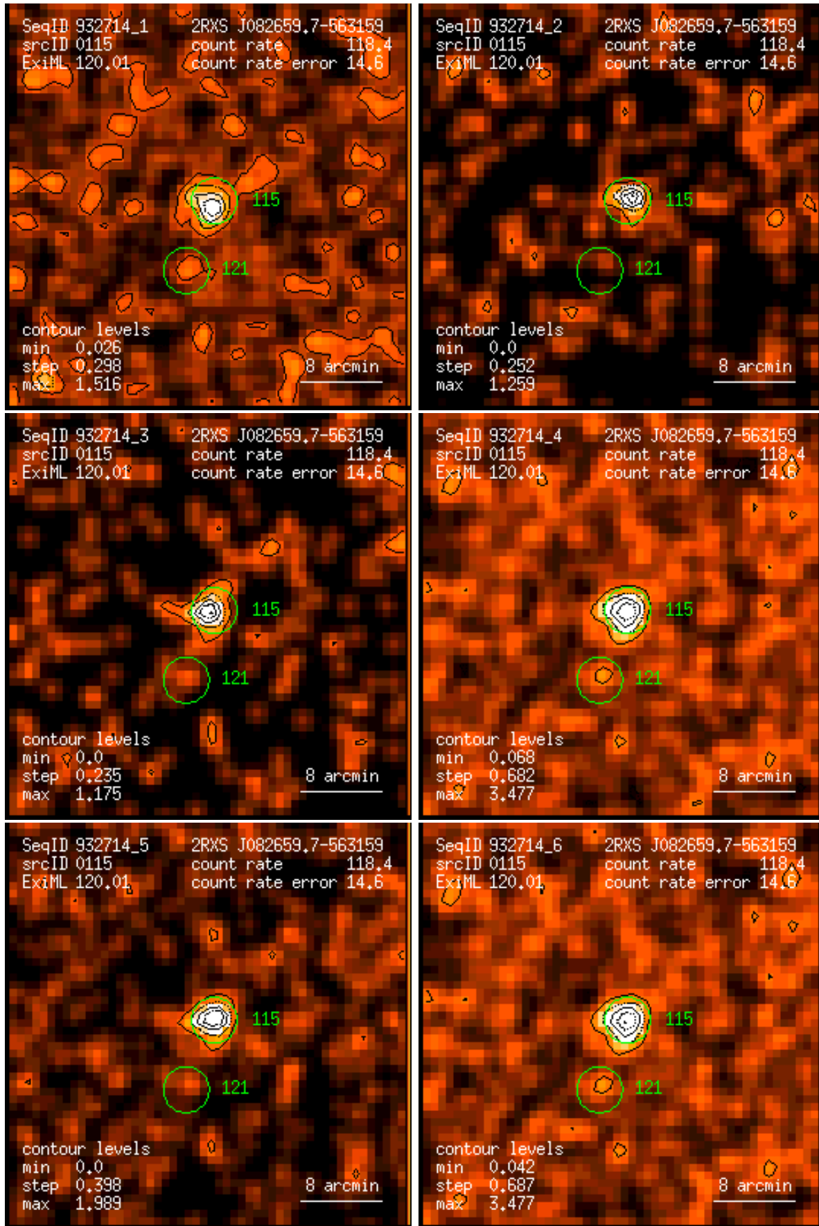
Figure 115: RASS 932714: detection 0115: band rate images, Gaussian filter: (1) PSPC channels 11 – 41, (2) 52 – 90, (3) 91 – 201, (4) 11 – 235, (5) 52 – 201, (6) 11 – 201. Broad band rates in counts/ks. Band rate contour levels in counts/ks/arcmin 2 .
