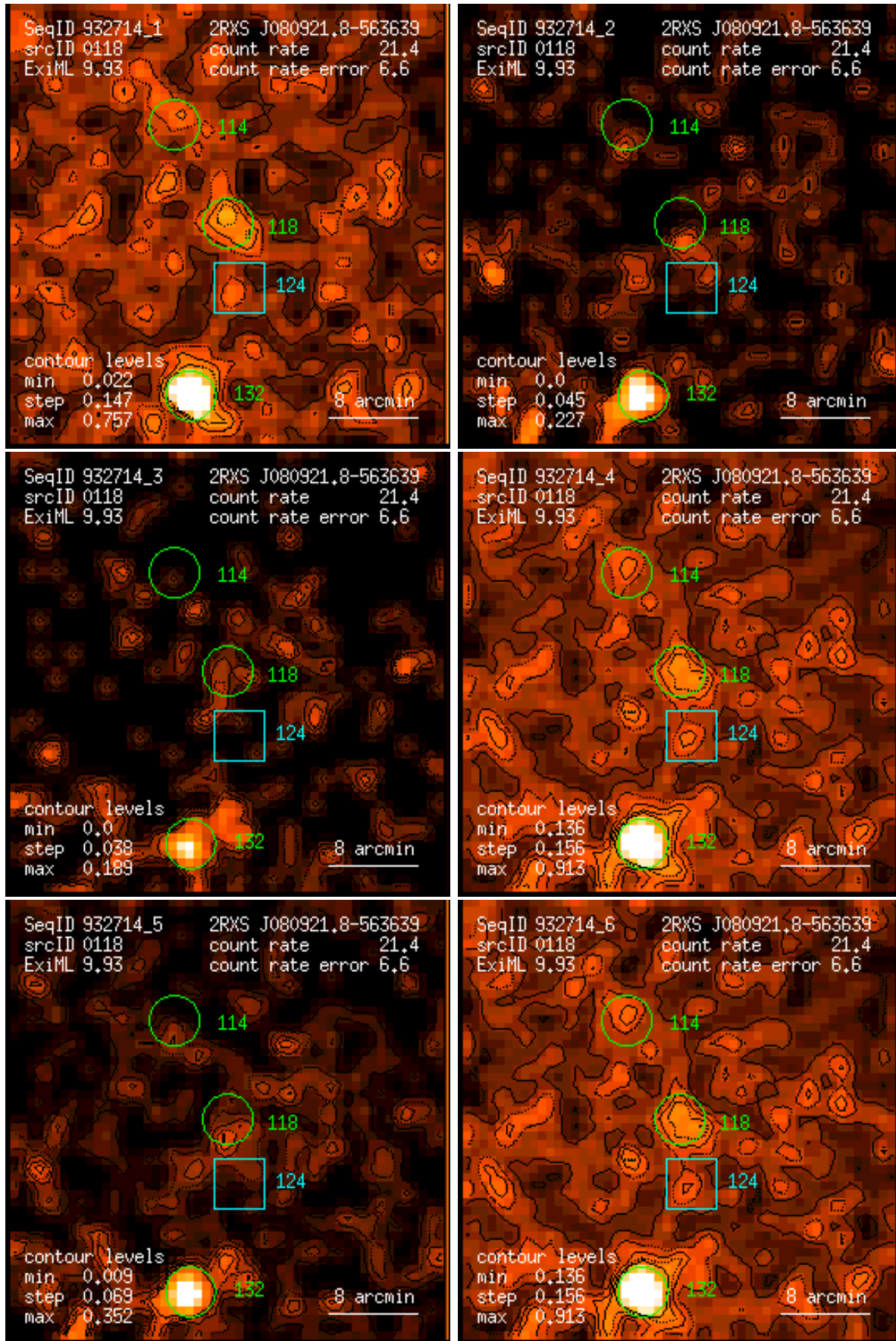
Figure 118: RASS 932714: detection 0118: band rate images, Gaussian filter: (1) PSPC channels 11 – 41, (2) 52 – 90, (3) 91 – 201, (4) 11 – 235, (5) 52 – 201, (6) 11 – 201. Broad band rates in counts/ks. Band rate contour levels in counts/ks/arcmin 2 .
