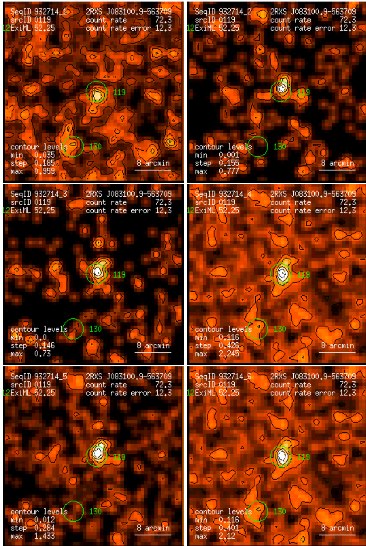
Figure 119: RASS 932714: detection 0119: band rate images, Gaussian filter: (1) PSPC channels 11 – 41, (2) 52 – 90, (3) 91 – 201, (4) 11 – 235, (5) 52 – 201, (6) 11 – 201. Broad band rates in counts/ks. Band rate contour levels in counts/ks/arcmin 2 .
