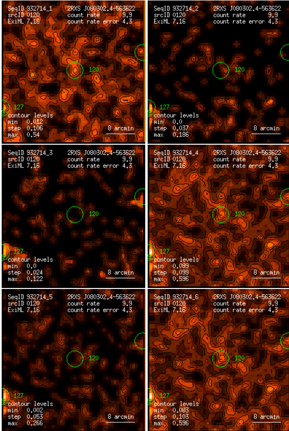
Figure 120: RASS 932714: detection 0120: band rate images, Gaussian filter: (1) PSPC channels 11 – 41, (2) 52 – 90, (3) 91 – 201, (4) 11 – 235, (5) 52 – 201, (6) 11 – 201. Broad band rates in counts/ks. Band rate contour levels in counts/ks/arcmin 2 .
