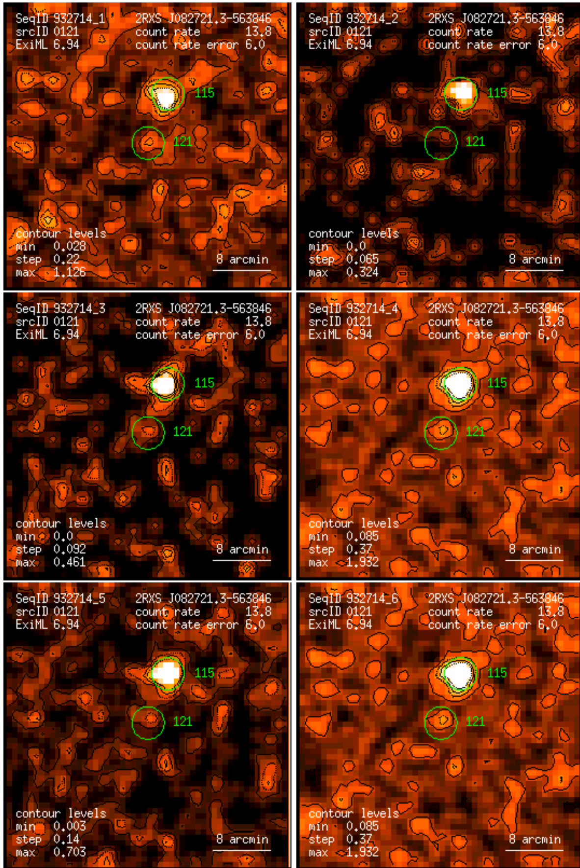
Figure 121: RASS 932714: detection 0121: band rate images, Gaussian filter: (1) PSPC channels 11 – 41, (2) 52 – 90, (3) 91 – 201, (4) 11 – 235, (5) 52 – 201, (6) 11 – 201. Broad band rates in counts/ks. Band rate contour levels in counts/ks/arcmin 2 .
