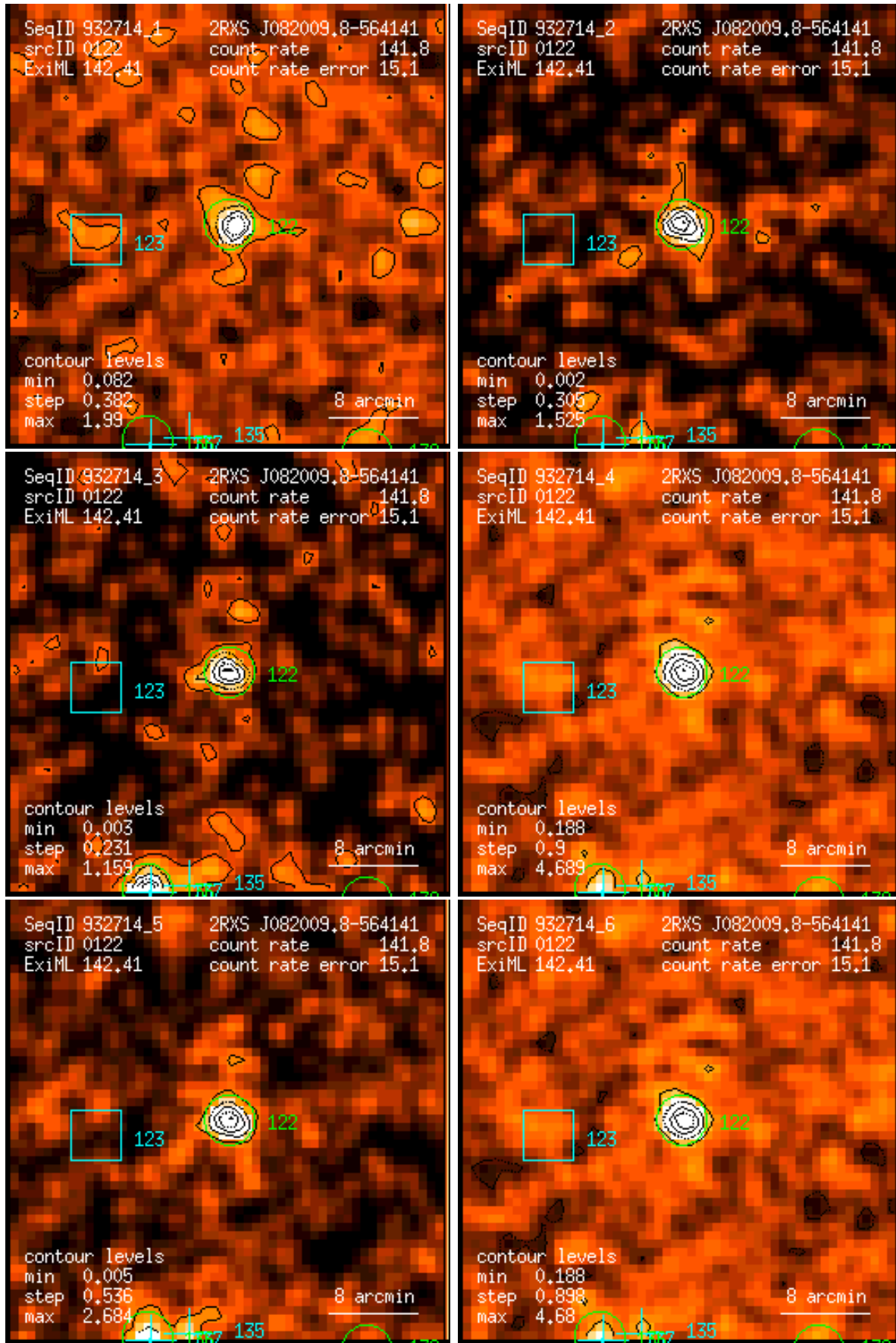
Figure 122: RASS 932714: detection 0122: band rate images, Gaussian filter: (1) PSPC channels 11 – 41, (2) 52 – 90, (3) 91 – 201, (4) 11 – 235, (5) 52 – 201, (6) 11 – 201. Broad band rates in counts/ks. Band rate contour levels in counts/ks/arcmin 2 .
