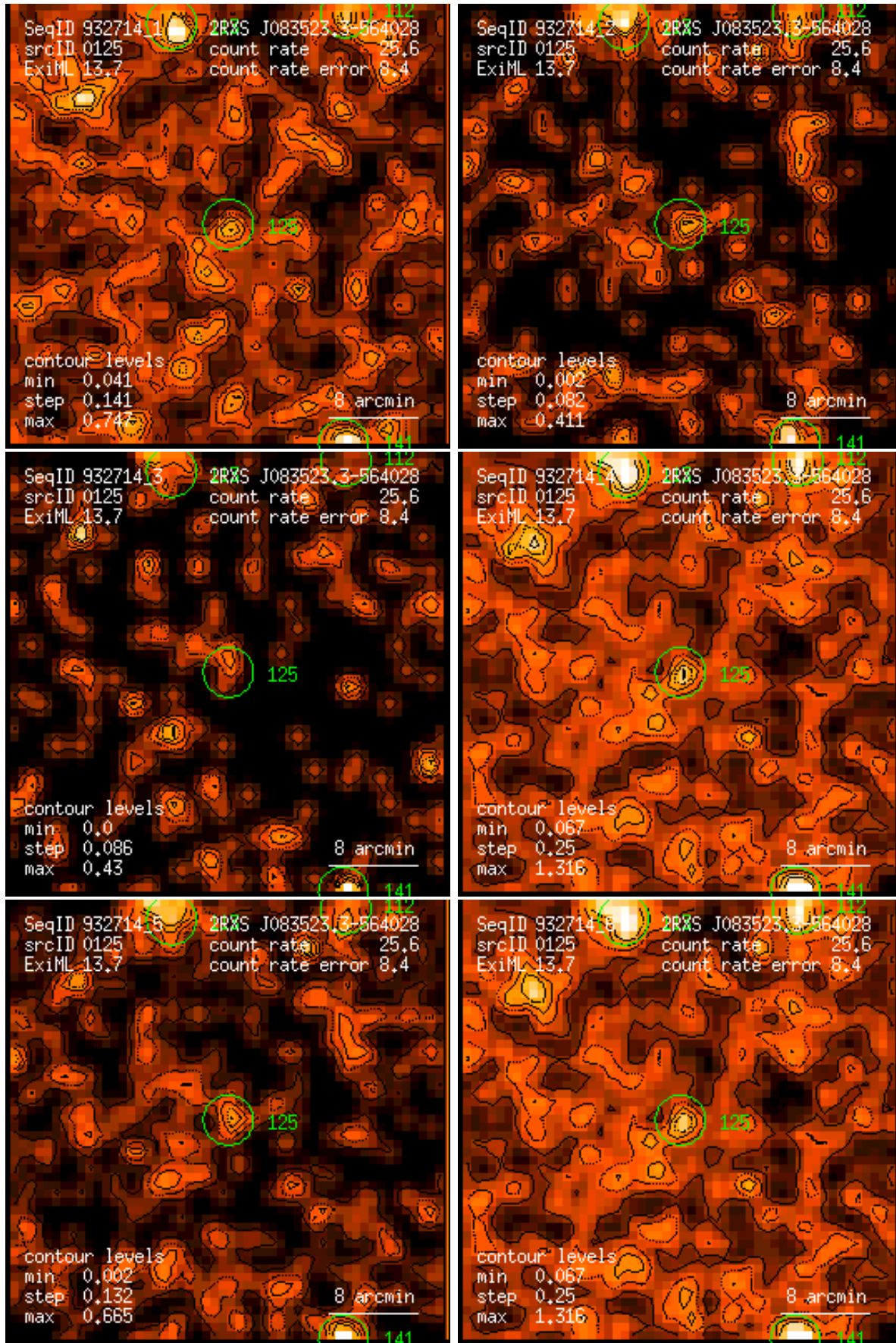
Figure 125: RASS 932714: detection 0125: band rate images, Gaussian filter: (1) PSPC channels 11 – 41, (2) 52 – 90, (3) 91 – 201, (4) 11 – 235, (5) 52 – 201, (6) 11 – 201. Broad band rates in counts/ks. Band rate contour levels in counts/ks/arcmin 2 .
