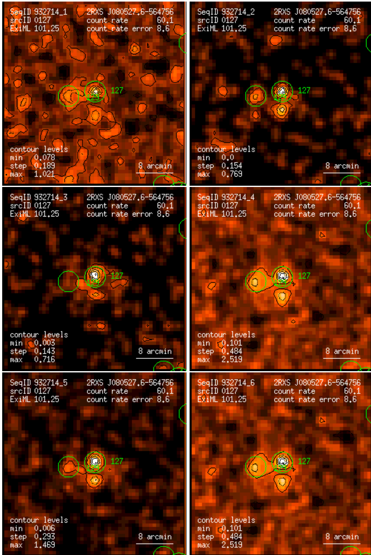
Figure 127: RASS 932714: detection 0127: band rate images, Gaussian filter: (1) PSPC channels 11 – 41, (2) 52 – 90, (3) 91 – 201, (4) 11 – 235, (5) 52 – 201, (6) 11 – 201. Broad band rates in counts/ks. Band rate contour levels in counts/ks/arcmin 2 .
