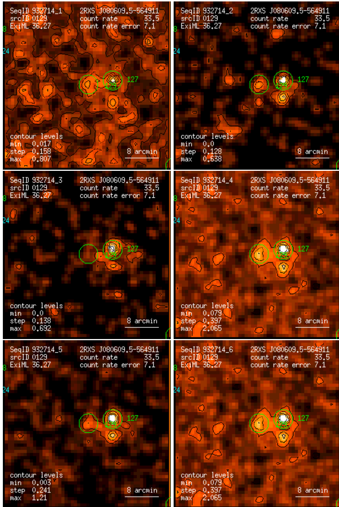
Figure 129: RASS 932714: detection 0129: band rate images, Gaussian filter: (1) PSPC channels 11 – 41, (2) 52 – 90, (3) 91 – 201, (4) 11 – 235, (5) 52 – 201, (6) 11 – 201. Broad band rates in counts/ks. Band rate contour levels in counts/ks/arcmin 2 .
