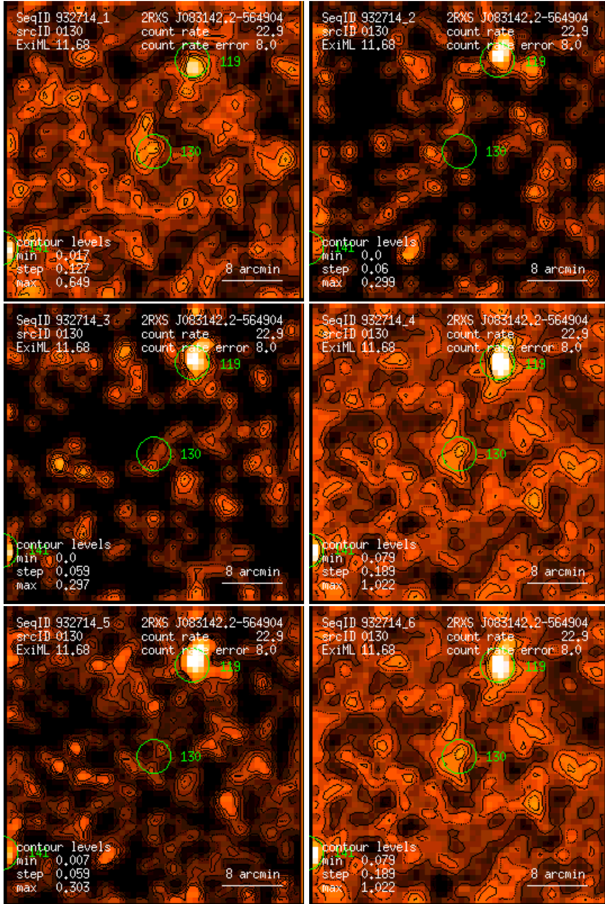
Figure 130: RASS 932714: detection 0130: band rate images, Gaussian filter: (1) PSPC channels 11 – 41, (2) 52 – 90, (3) 91 – 201, (4) 11 – 235, (5) 52 – 201, (6) 11 – 201. Broad band rates in counts/ks. Band rate contour levels in counts/ks/arcmin 2 .
