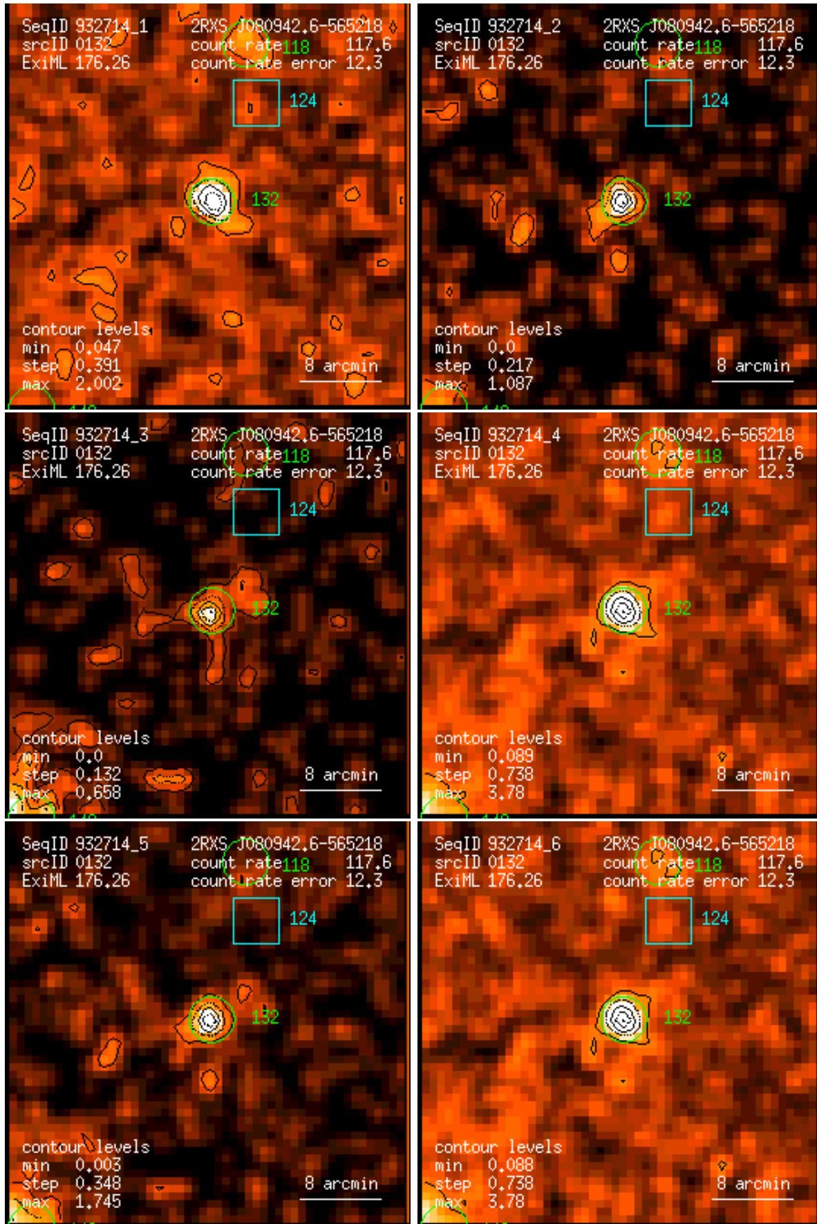
Figure 132: RASS 932714: detection 0132: band rate images, Gaussian filter: (1) PSPC channels 11 – 41, (2) 52 – 90, (3) 91 – 201, (4) 11 – 235, (5) 52 – 201, (6) 11 – 201. Broad band rates in counts/ks. Band rate contour levels in counts/ks/arcmin 2 .
