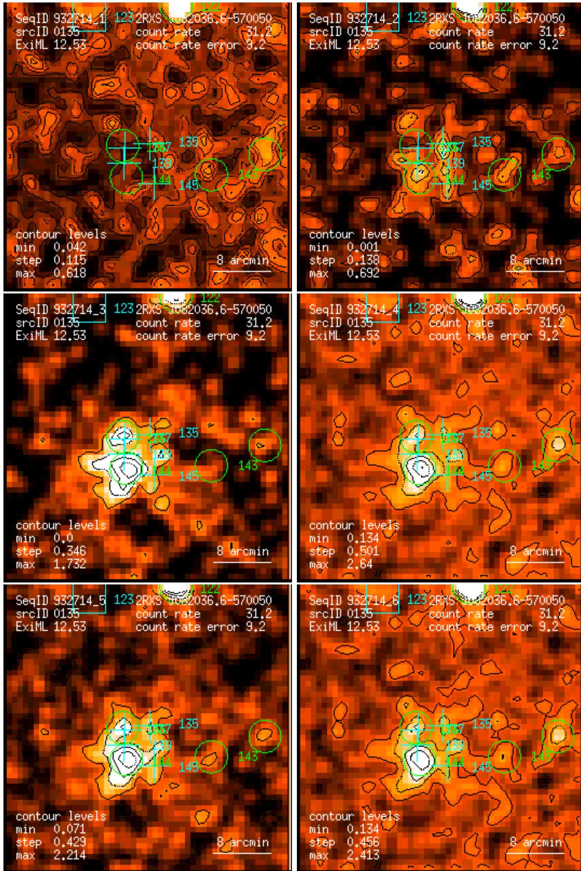
Figure 135: RASS 932714: detection 0135: band rate images, Gaussian filter: (1) PSPC channels 11 – 41, (2) 52 – 90, (3) 91 – 201, (4) 11 – 235, (5) 52 – 201, (6) 11 – 201. Broad band rates in counts/ks. Band rate contour levels in counts/ks/arcmin 2 .
