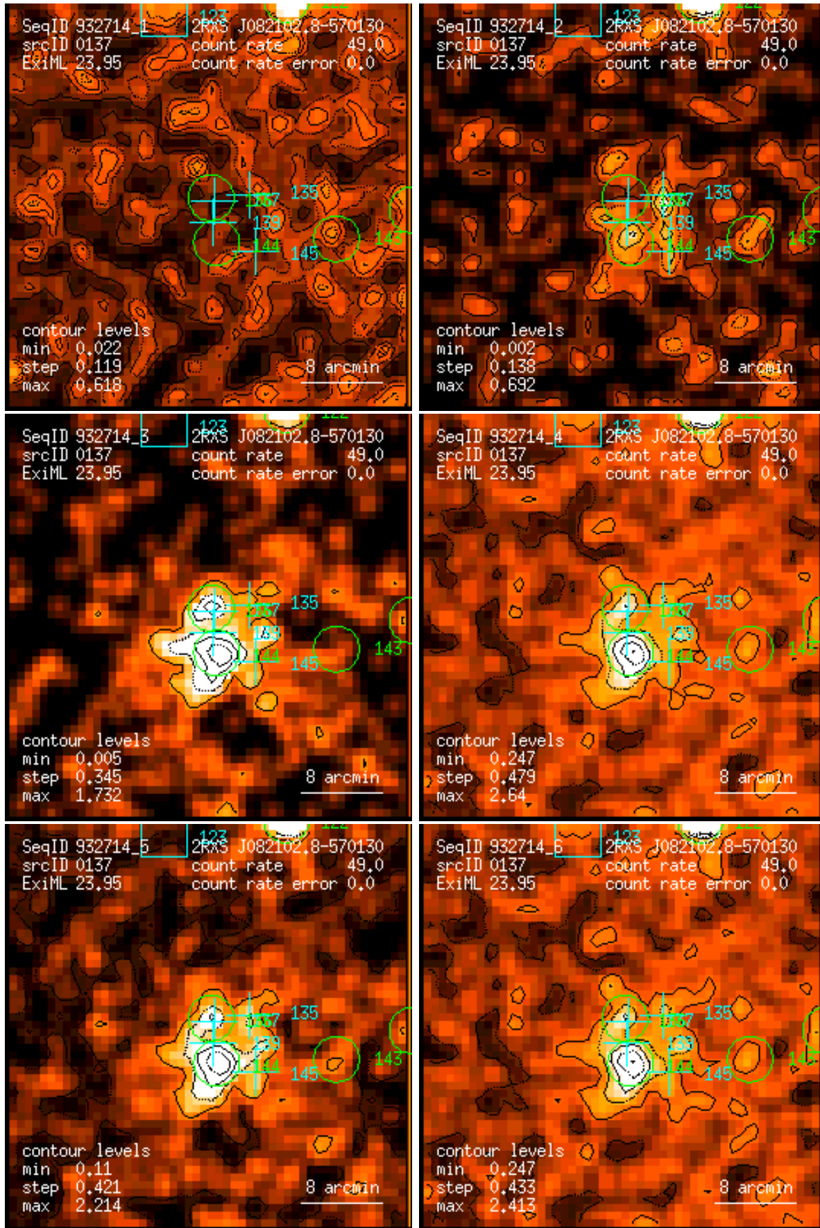
Figure 137: RASS 932714: detection 0137: band rate images, Gaussian filter: (1) PSPC channels 11 – 41, (2) 52 – 90, (3) 91 – 201, (4) 11 – 235, (5) 52 – 201, (6) 11 – 201. Broad band rates in counts/ks. Band rate contour levels in counts/ks/arcmin 2 .
