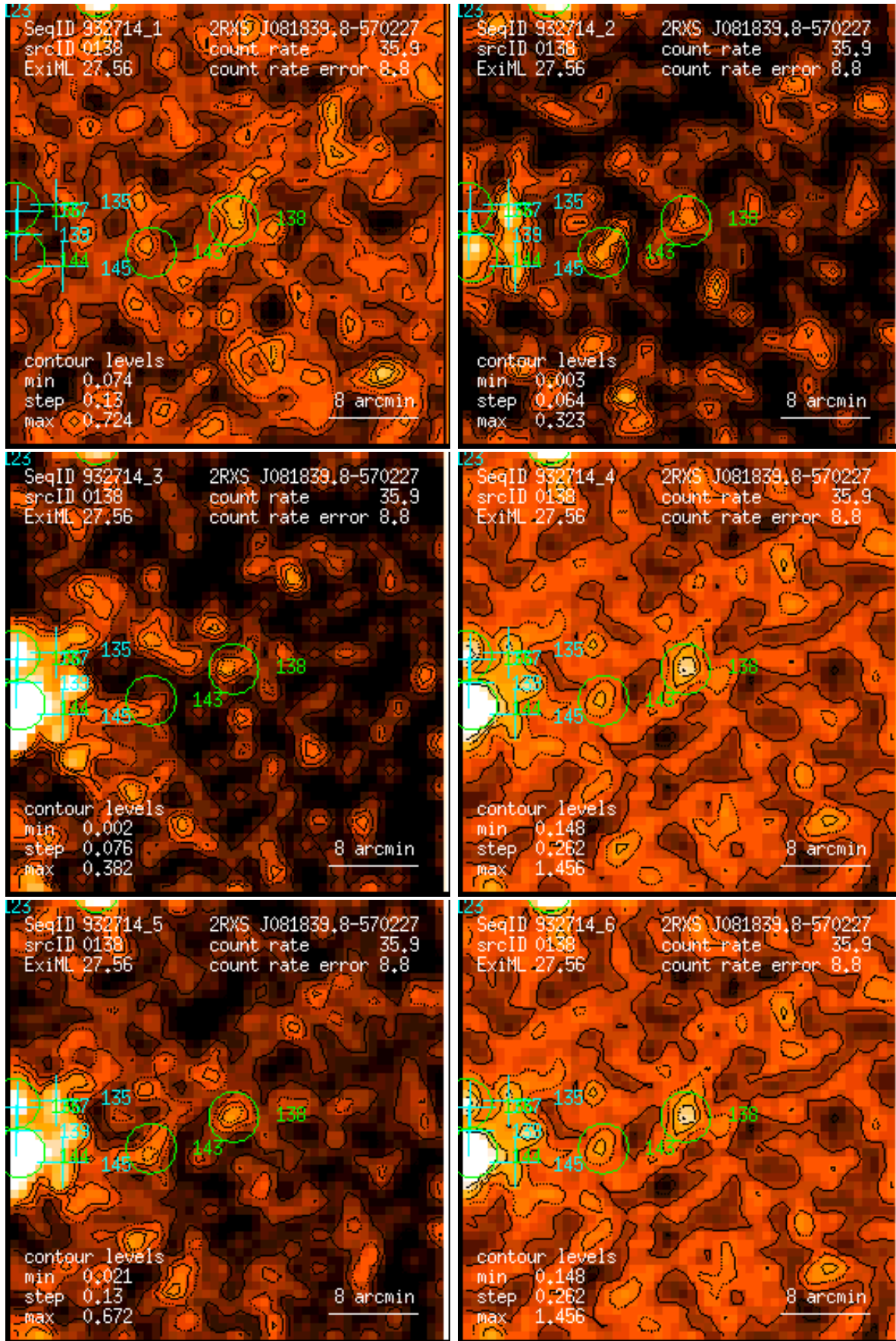
Figure 138: RASS 932714: detection 0138: band rate images, Gaussian filter: (1) PSPC channels 11 – 41, (2) 52 – 90, (3) 91 – 201, (4) 11 – 235, (5) 52 – 201, (6) 11 – 201. Broad band rates in counts/ks. Band rate contour levels in counts/ks/arcmin 2 .
