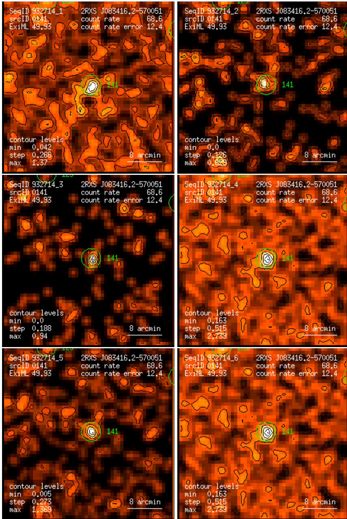
Figure 141: RASS 932714: detection 0141: band rate images, Gaussian filter: (1) PSPC channels 11 – 41, (2) 52 – 90, (3) 91 – 201, (4) 11 – 235, (5) 52 – 201, (6) 11 – 201. Broad band rates in counts/ks. Band rate contour levels in counts/ks/arcmin 2 .
