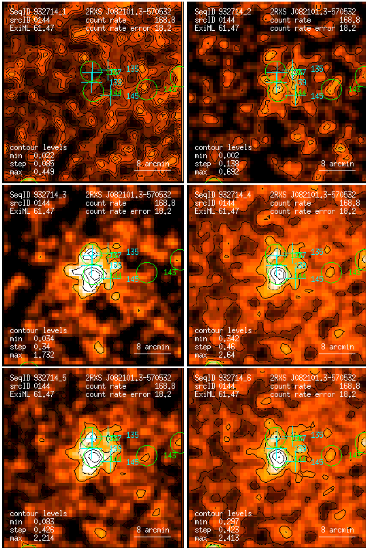
Figure 144: RASS 932714: detection 0144: band rate images, Gaussian filter: (1) PSPC channels 11 – 41, (2) 52 – 90, (3) 91 – 201, (4) 11 – 235, (5) 52 – 201, (6) 11 – 201. Broad band rates in counts/ks. Band rate contour levels in counts/ks/arcmin 2 .
