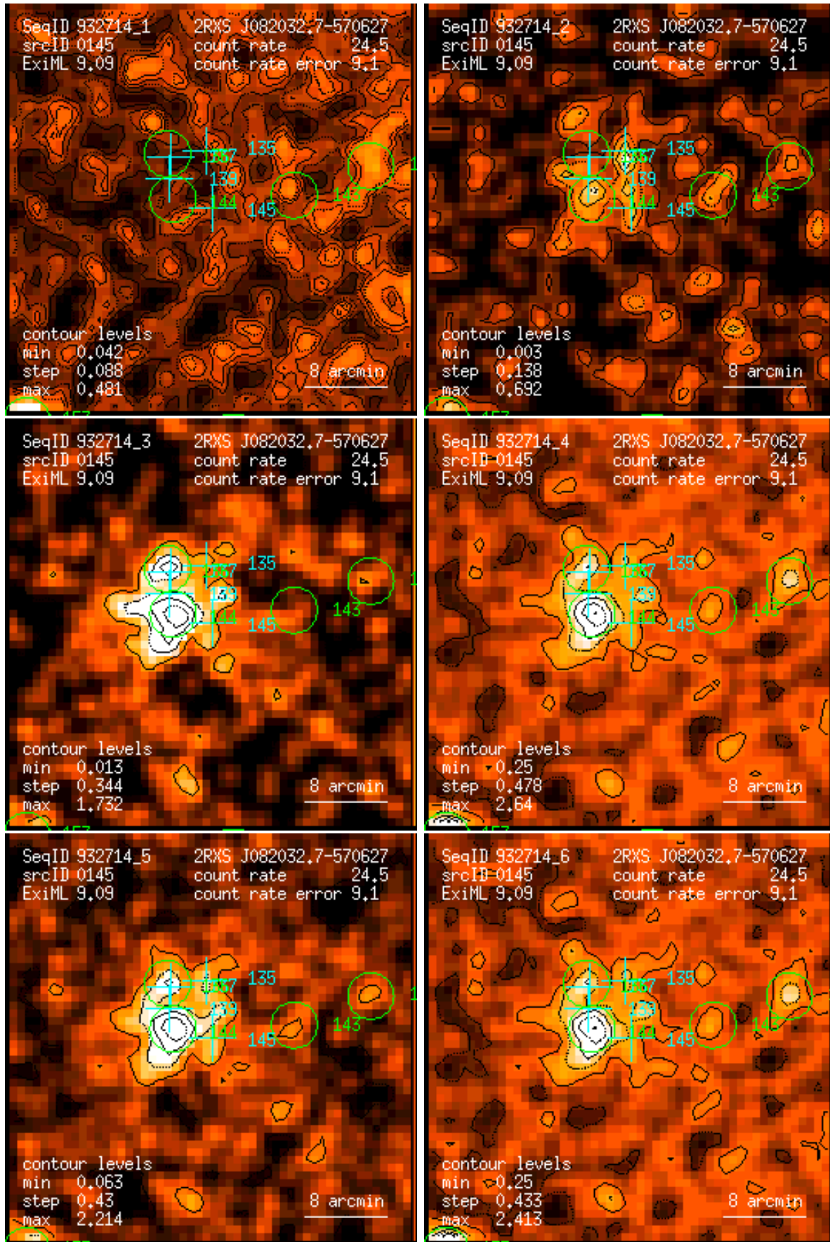
Figure 145: RASS 932714: detection 0145: band rate images, Gaussian filter: (1) PSPC channels 11 – 41, (2) 52 – 90, (3) 91 – 201, (4) 11 – 235, (5) 52 – 201, (6) 11 – 201. Broad band rates in counts/ks. Band rate contour levels in counts/ks/arcmin 2 .
