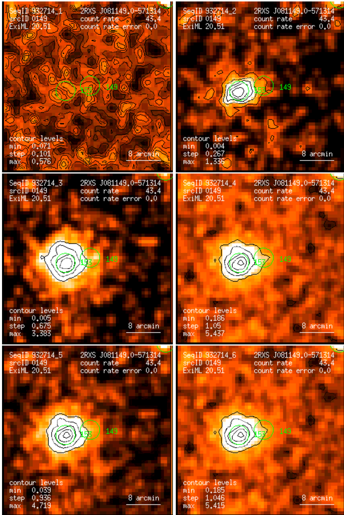
Figure 149: RASS 932714: detection 0149: band rate images, Gaussian filter: (1) PSPC channels 11 – 41, (2) 52 – 90, (3) 91 – 201, (4) 11 – 235, (5) 52 – 201, (6) 11 – 201. Broad band rates in counts/ks. Band rate contour levels in counts/ks/arcmin 2 .
