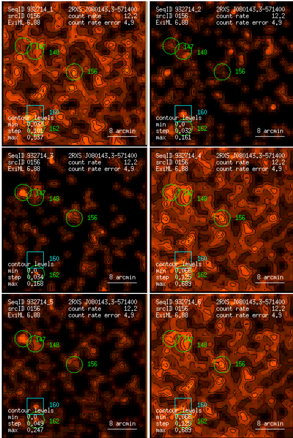
Figure 156: RASS 932714: detection 0156: band rate images, Gaussian filter: (1) PSPC channels 11 – 41, (2) 52 – 90, (3) 91 – 201, (4) 11 – 235, (5) 52 – 201, (6) 11 – 201. Broad band rates in counts/ks. Band rate contour levels in counts/ks/arcmin 2 .
