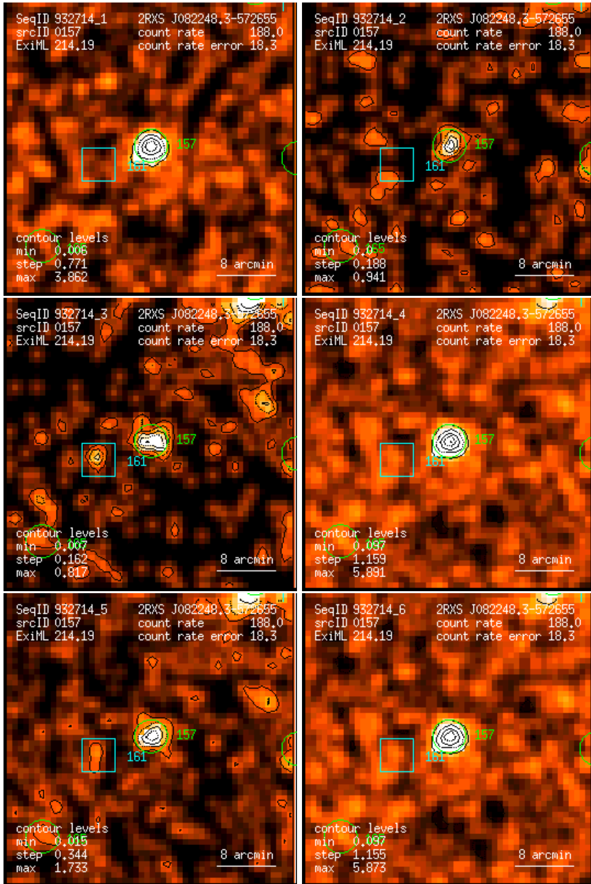
Figure 157: RASS 932714: detection 0157: band rate images, Gaussian filter: (1) PSPC channels 11 – 41, (2) 52 – 90, (3) 91 – 201, (4) 11 – 235, (5) 52 – 201, (6) 11 – 201. Broad band rates in counts/ks. Band rate contour levels in counts/ks/arcmin 2 .
