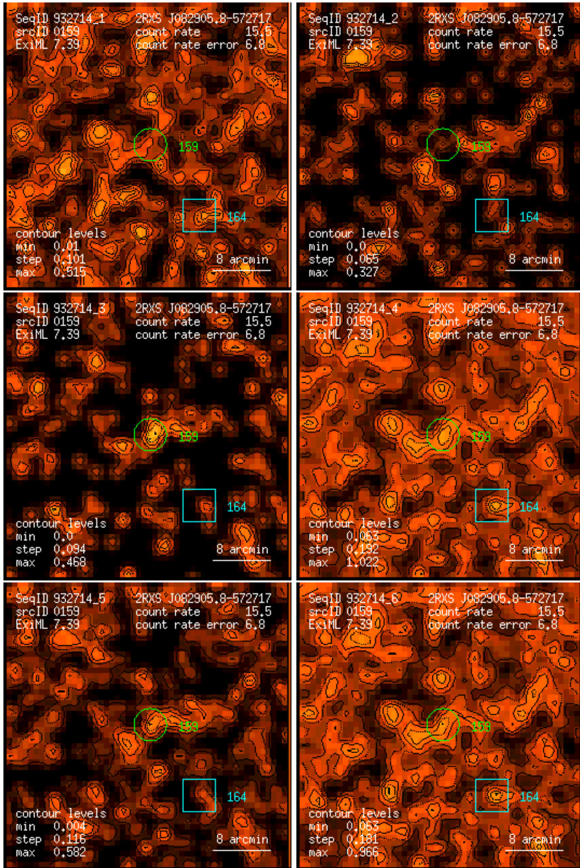
Figure 159: RASS 932714: detection 0159: band rate images, Gaussian filter: (1) PSPC channels 11 – 41, (2) 52 – 90, (3) 91 – 201, (4) 11 – 235, (5) 52 – 201, (6) 11 – 201. Broad band rates in counts/ks. Band rate contour levels in counts/ks/arcmin 2 .
