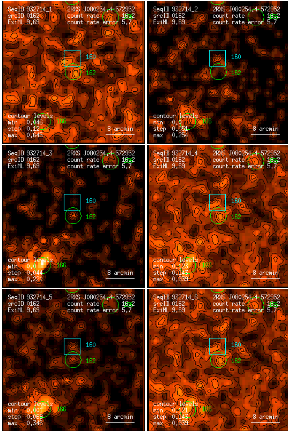
Figure 162: RASS 932714: detection 0162: band rate images, Gaussian filter: (1) PSPC channels 11 – 41, (2) 52 – 90, (3) 91 – 201, (4) 11 – 235, (5) 52 – 201, (6) 11 – 201. Broad band rates in counts/ks. Band rate contour levels in counts/ks/arcmin 2 .
