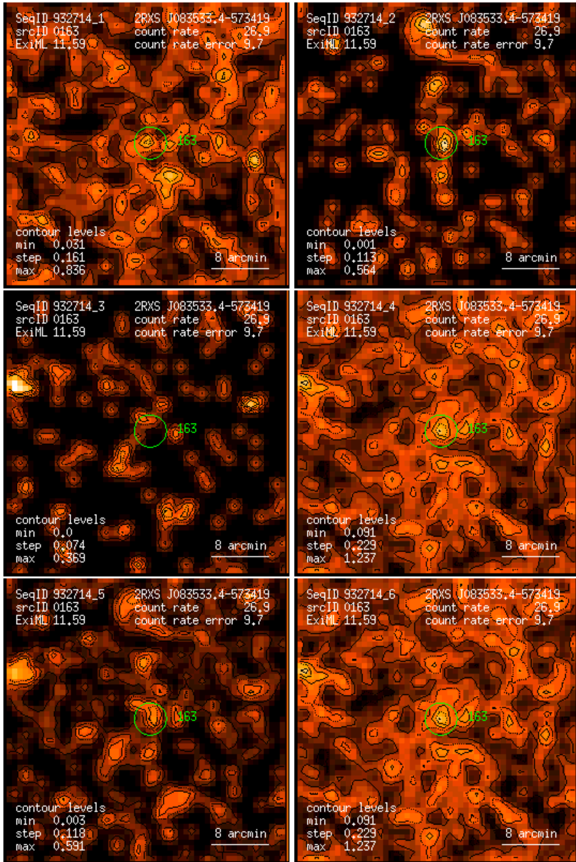
Figure 163: RASS 932714: detection 0163: band rate images, Gaussian filter: (1) PSPC channels 11 – 41, (2) 52 – 90, (3) 91 – 201, (4) 11 – 235, (5) 52 – 201, (6) 11 – 201. Broad band rates in counts/ks. Band rate contour levels in counts/ks/arcmin 2 .
