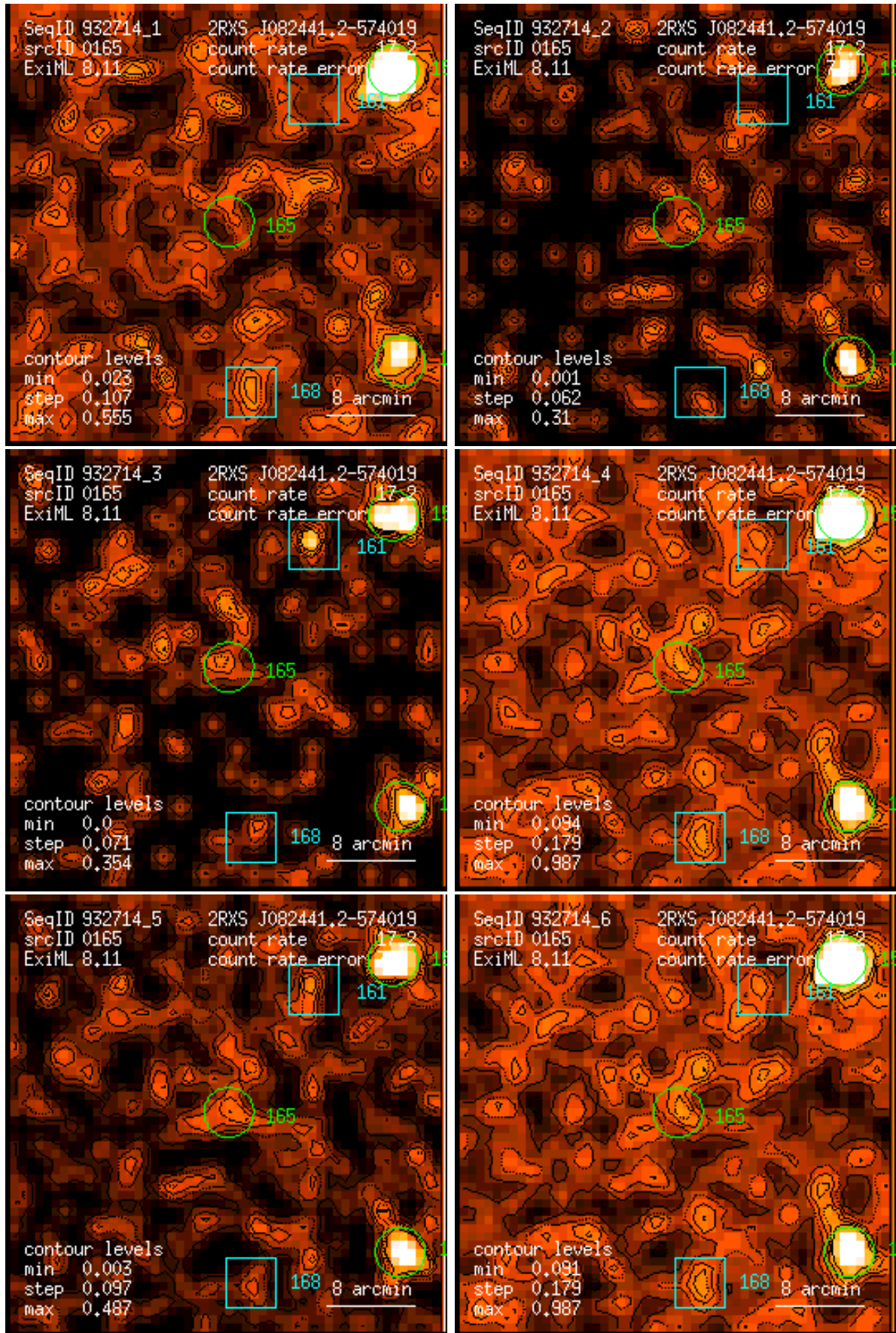
Figure 165: RASS 932714: detection 0165: band rate images, Gaussian filter: (1) PSPC channels 11 – 41, (2) 52 – 90, (3) 91 – 201, (4) 11 – 235, (5) 52 – 201, (6) 11 – 201. Broad band rates in counts/ks. Band rate contour levels in counts/ks/arcmin 2 .
