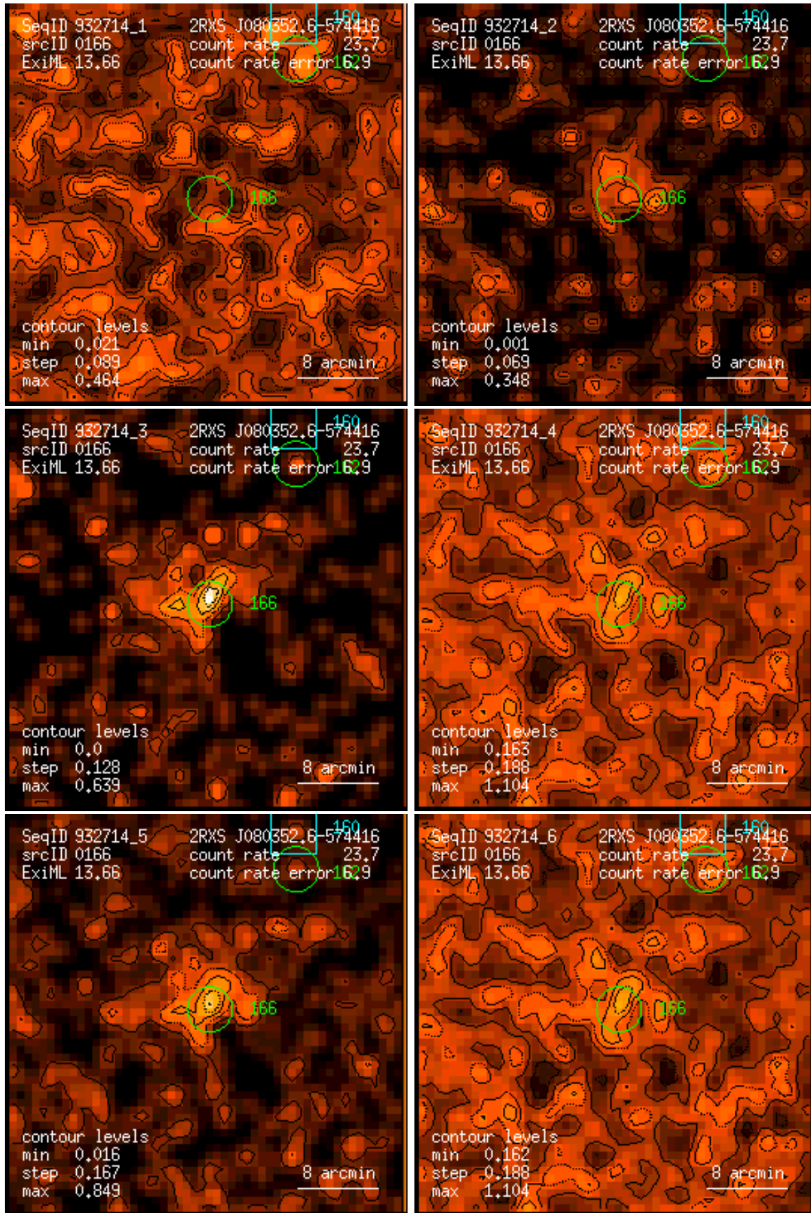
Figure 166: RASS 932714: detection 0166: band rate images, Gaussian filter: (1) PSPC channels 11 – 41, (2) 52 – 90, (3) 91 – 201, (4) 11 – 235, (5) 52 – 201, (6) 11 – 201. Broad band rates in counts/ks. Band rate contour levels in counts/ks/arcmin 2 .
