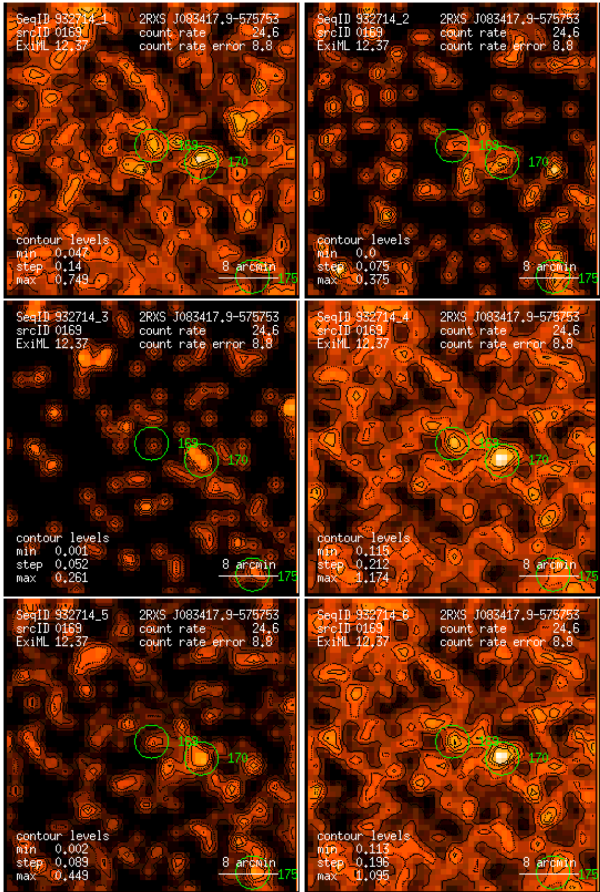
Figure 169: RASS 932714: detection 0169: band rate images, Gaussian filter: (1) PSPC channels 11 – 41, (2) 52 – 90, (3) 91 – 201, (4) 11 – 235, (5) 52 – 201, (6) 11 – 201. Broad band rates in counts/ks. Band rate contour levels in counts/ks/arcmin 2 .
