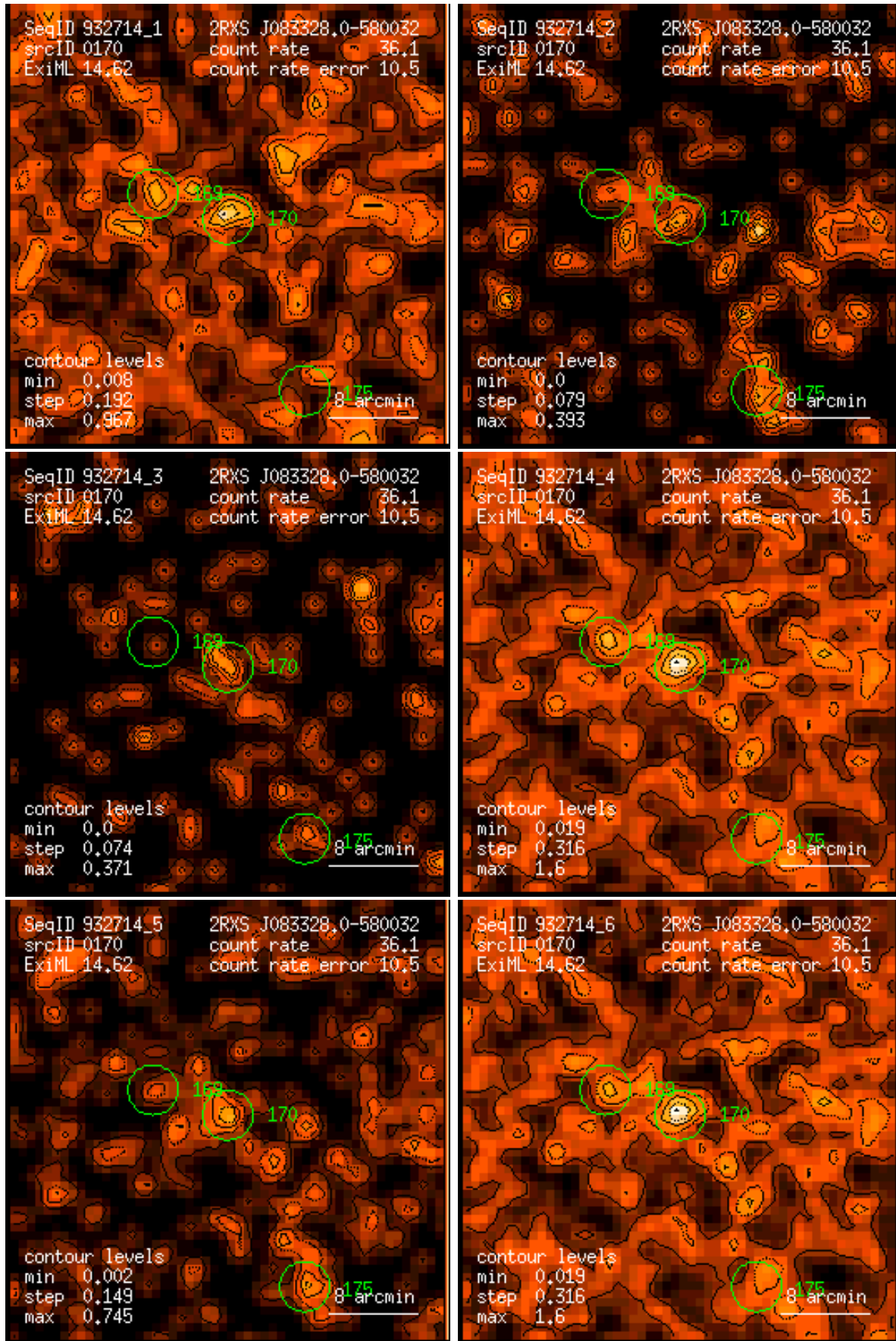
Figure 170: RASS 932714: detection 0170: band rate images, Gaussian filter: (1) PSPC channels 11 – 41, (2) 52 – 90, (3) 91 – 201, (4) 11 – 235, (5) 52 – 201, (6) 11 – 201. Broad band rates in counts/ks. Band rate contour levels in counts/ks/arcmin 2 .
