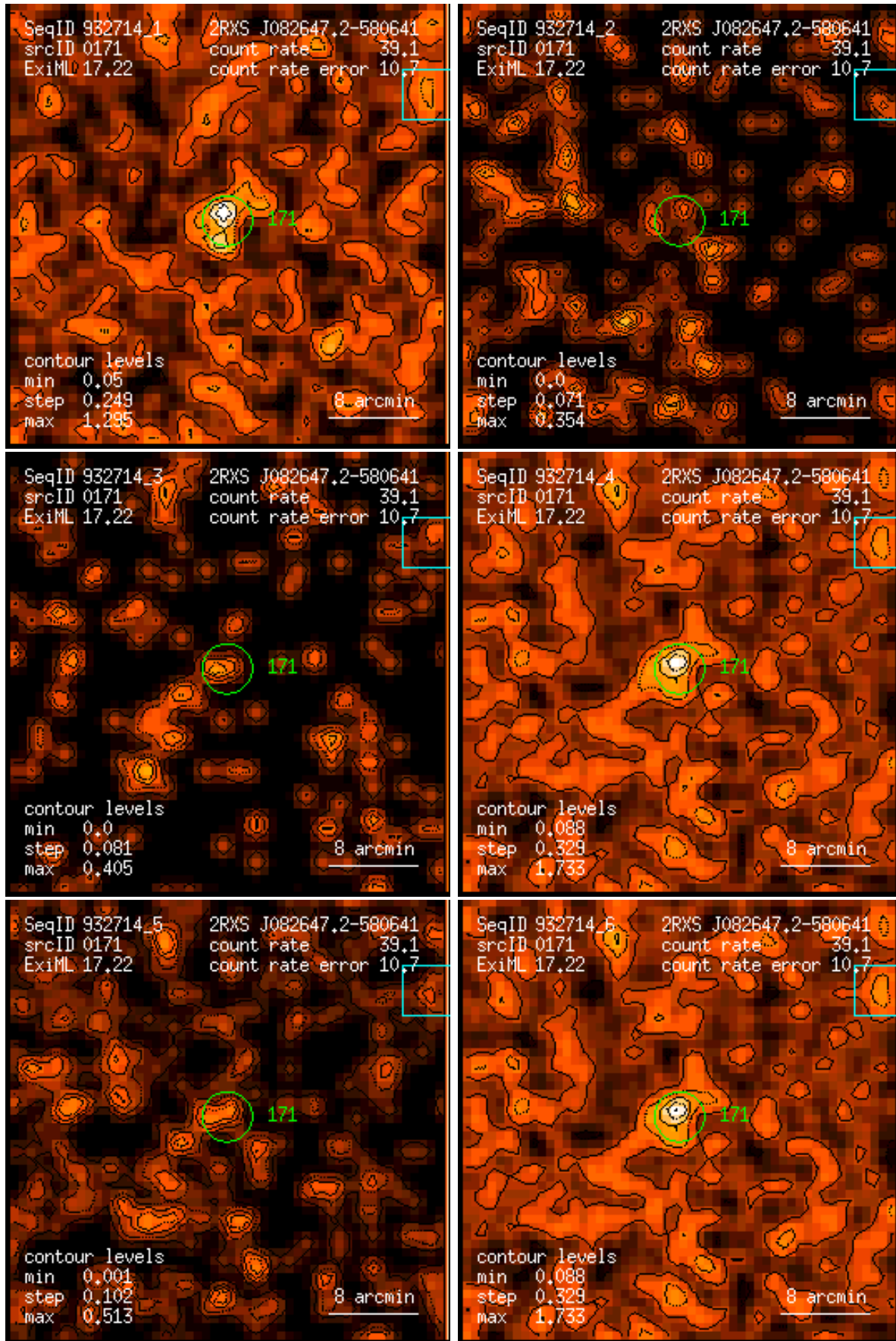
Figure 171: RASS 932714: detection 0171: band rate images, Gaussian filter: (1) PSPC channels 11 – 41, (2) 52 – 90, (3) 91 – 201, (4) 11 – 235, (5) 52 – 201, (6) 11 – 201. Broad band rates in counts/ks. Band rate contour levels in counts/ks/arcmin 2 .
