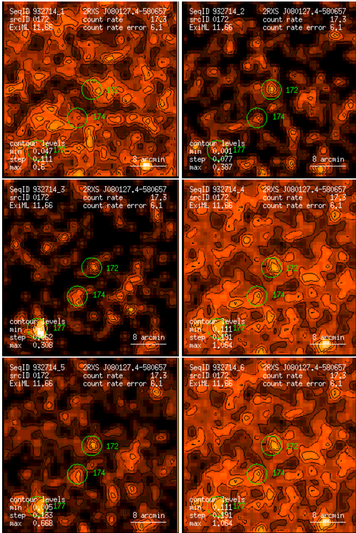
Figure 172: RASS 932714: detection 0172: band rate images, Gaussian filter: (1) PSPC channels 11 – 41, (2) 52 – 90, (3) 91 – 201, (4) 11 – 235, (5) 52 – 201, (6) 11 – 201. Broad band rates in counts/ks. Band rate contour levels in counts/ks/arcmin 2 .
