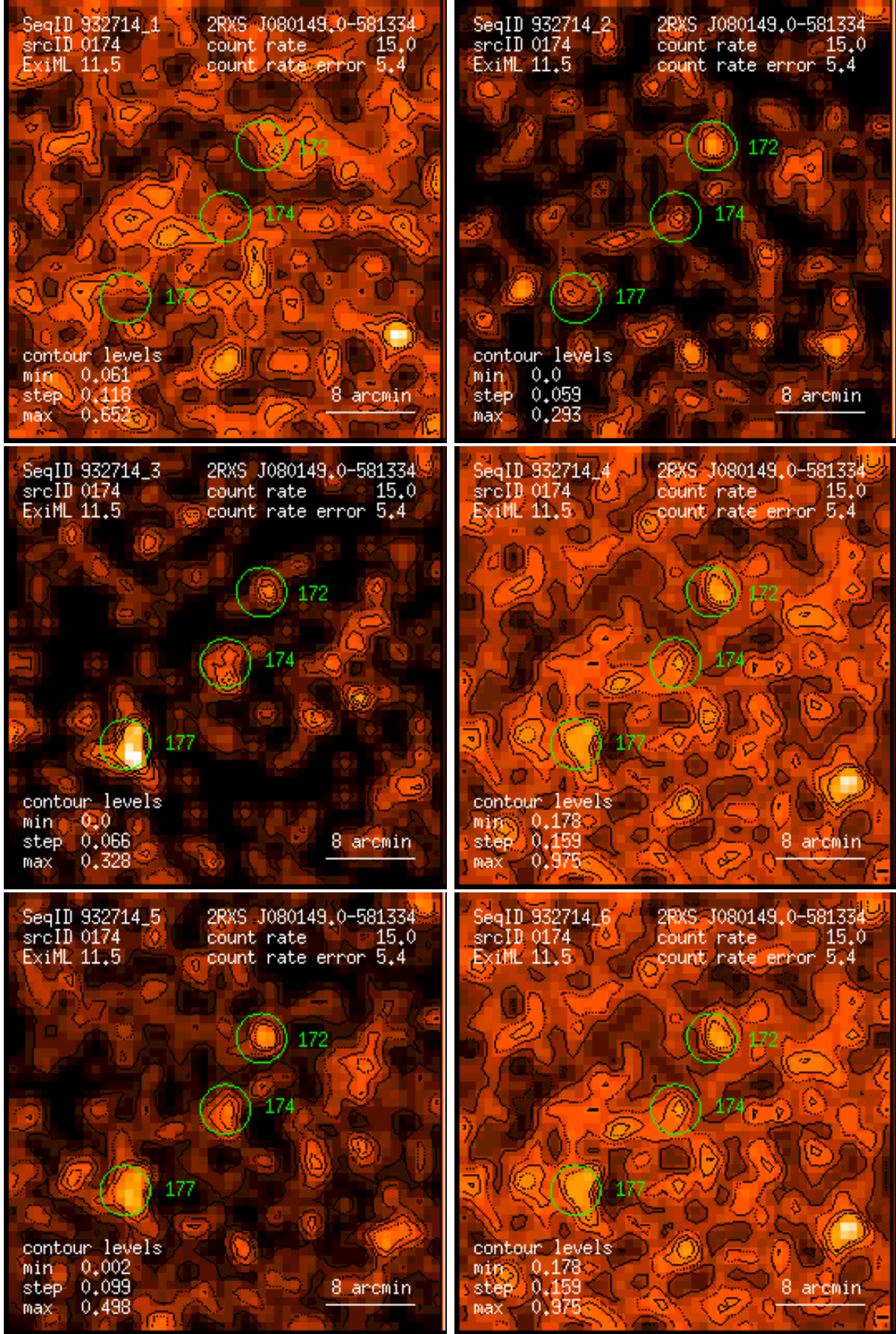
Figure 174: RASS 932714: detection 0174: band rate images, Gaussian filter: (1) PSPC channels 11 – 41, (2) 52 – 90, (3) 91 – 201, (4) 11 – 235, (5) 52 – 201, (6) 11 – 201. Broad band rates in counts/ks. Band rate contour levels in counts/ks/arcmin 2 .
