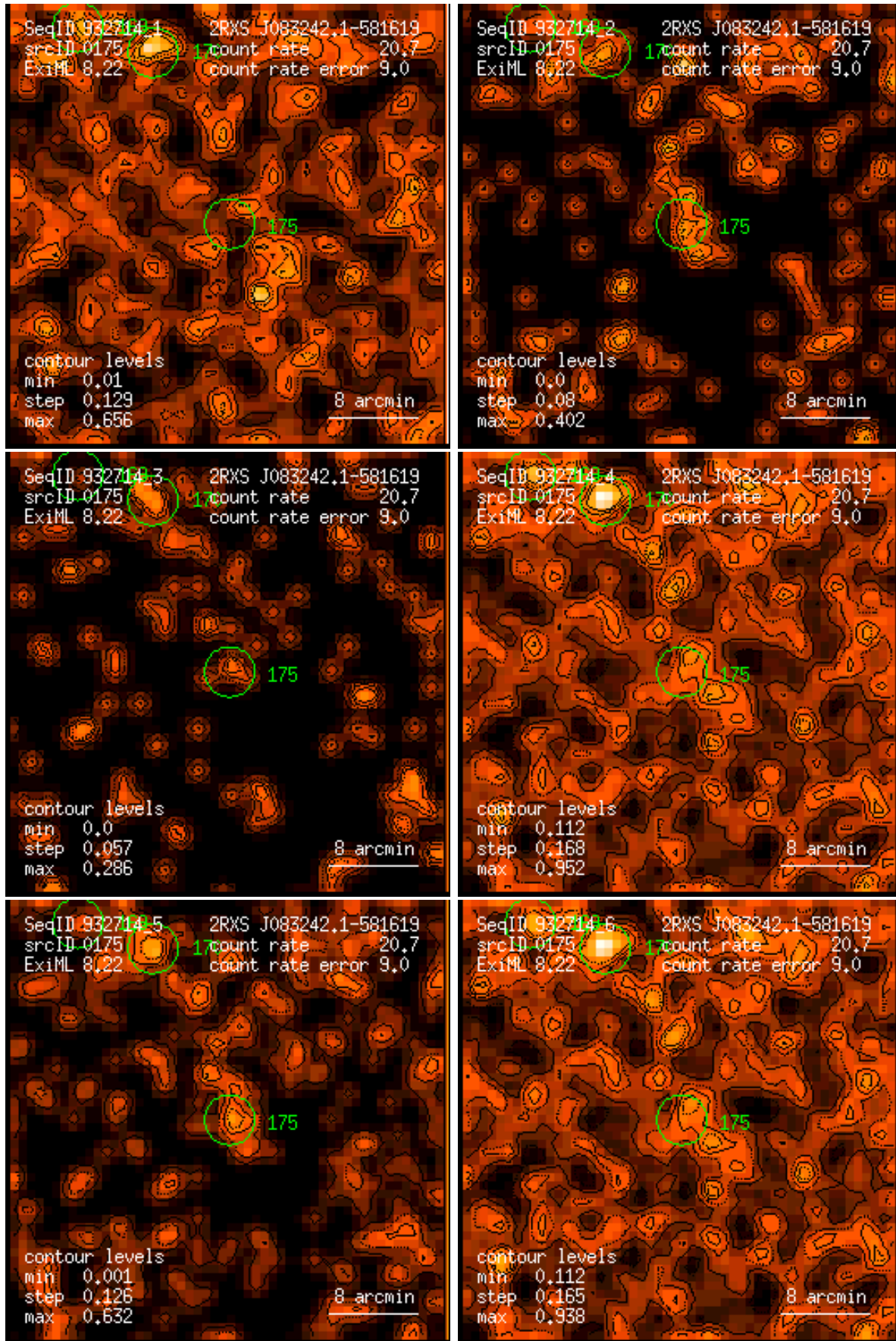
Figure 175: RASS 932714: detection 0175: band rate images, Gaussian filter: (1) PSPC channels 11 – 41, (2) 52 – 90, (3) 91 – 201, (4) 11 – 235, (5) 52 – 201, (6) 11 – 201. Broad band rates in counts/ks. Band rate contour levels in counts/ks/arcmin 2 .
