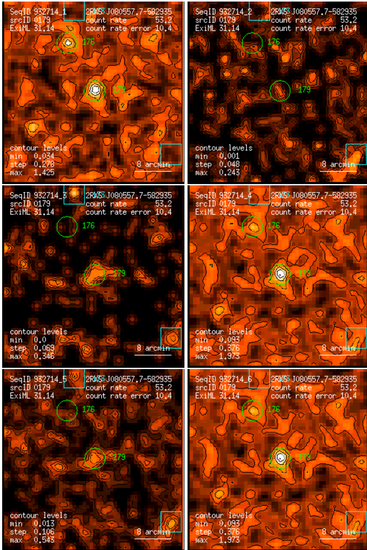
Figure 179: RASS 932714: detection 0179: band rate images, Gaussian filter: (1) PSPC channels 11 – 41, (2) 52 – 90, (3) 91 – 201, (4) 11 – 235, (5) 52 – 201, (6) 11 – 201. Broad band rates in counts/ks. Band rate contour levels in counts/ks/arcmin 2 .
