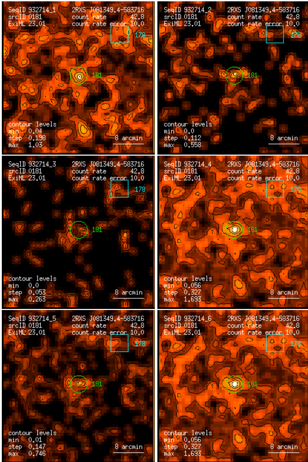
Figure 181: RASS 932714: detection 0181: band rate images, Gaussian filter: (1) PSPC channels 11 – 41, (2) 52 – 90, (3) 91 – 201, (4) 11 – 235, (5) 52 – 201, (6) 11 – 201. Broad band rates in counts/ks. Band rate contour levels in counts/ks/arcmin 2 .
