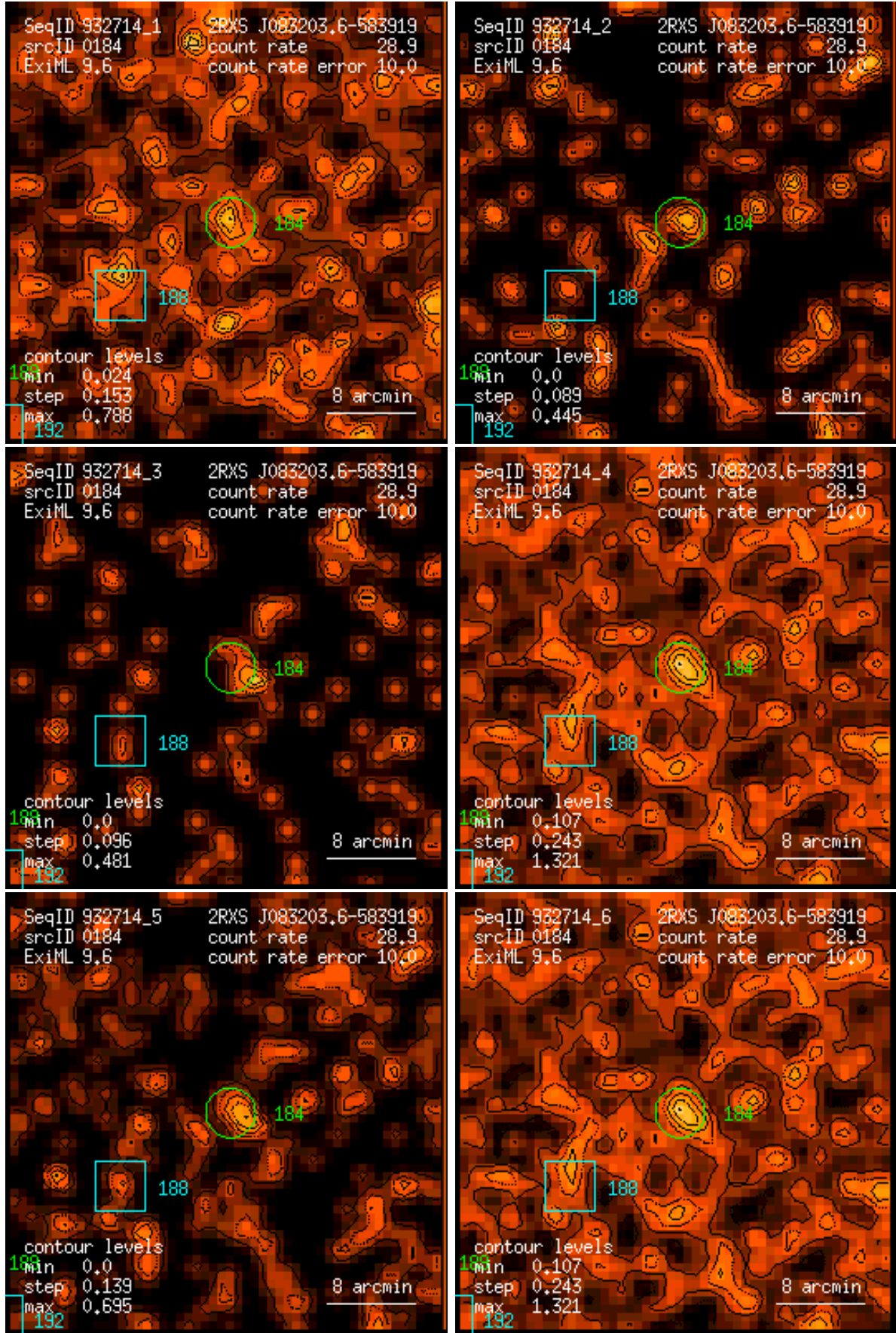
Figure 184: RASS 932714: detection 0184: band rate images, Gaussian filter: (1) PSPC channels 11 – 41, (2) 52 – 90, (3) 91 – 201, (4) 11 – 235, (5) 52 – 201, (6) 11 – 201. Broad band rates in counts/ks. Band rate contour levels in counts/ks/arcmin 2 .
