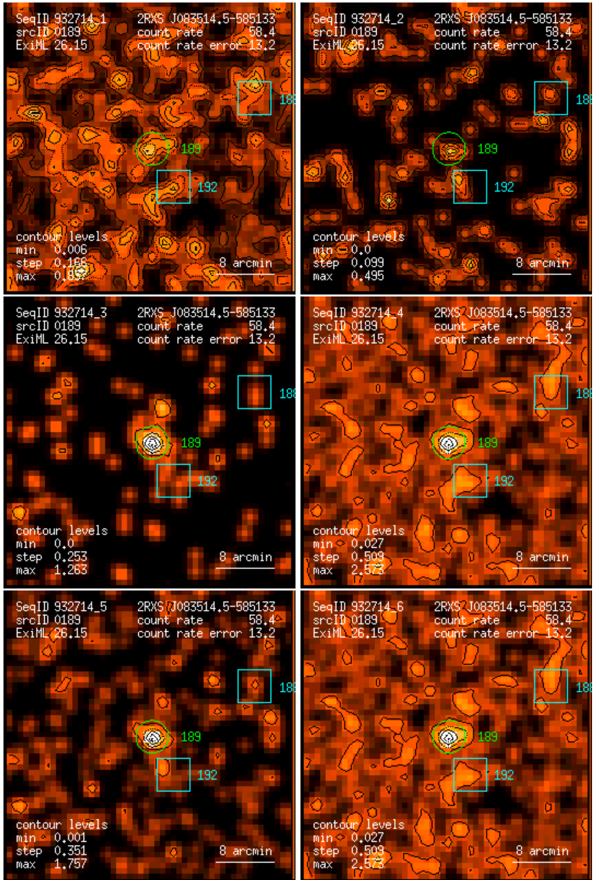
Figure 189: RASS 932714: detection 0189: band rate images, Gaussian filter: (1) PSPC channels 11 – 41, (2) 52 – 90, (3) 91 – 201, (4) 11 – 235, (5) 52 – 201, (6) 11 – 201. Broad band rates in counts/ks. Band rate contour levels in counts/ks/arcmin 2 .
