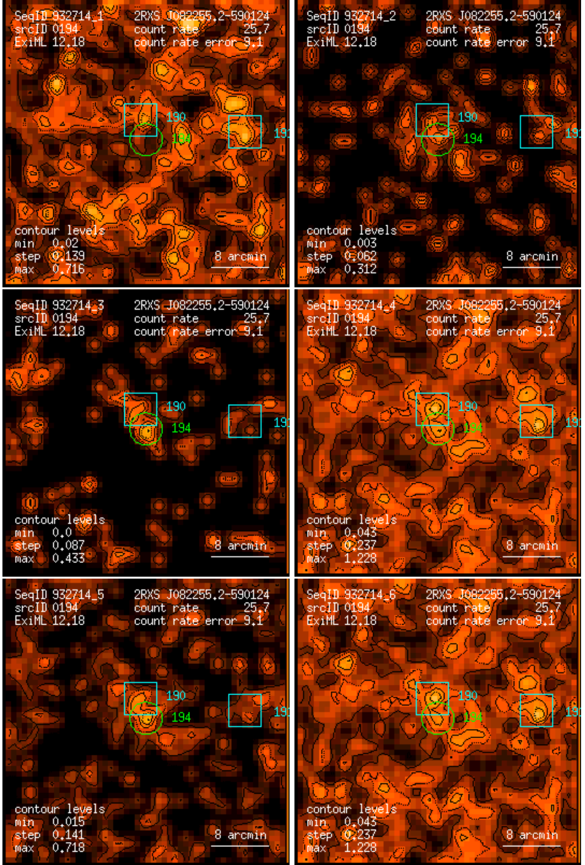
Figure 194: RASS 932714: detection 0194: band rate images, Gaussian filter: (1) PSPC channels 11 – 41, (2) 52 – 90, (3) 91 – 201, (4) 11 – 235, (5) 52 – 201, (6) 11 – 201. Broad band rates in counts/ks. Band rate contour levels in counts/ks/arcmin 2 .
