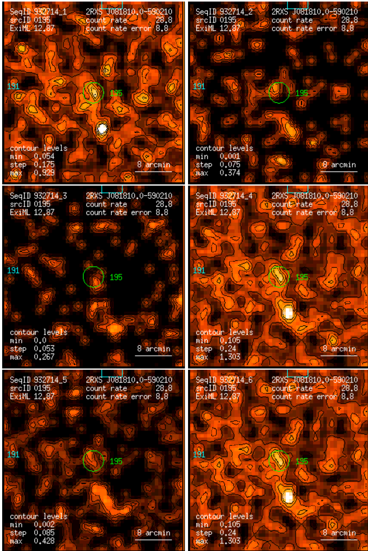
Figure 195: RASS 932714: detection 0195: band rate images, Gaussian filter: (1) PSPC channels 11 – 41, (2) 52 – 90, (3) 91 – 201, (4) 11 – 235, (5) 52 – 201, (6) 11 – 201. Broad band rates in counts/ks. Band rate contour levels in counts/ks/arcmin 2 .
