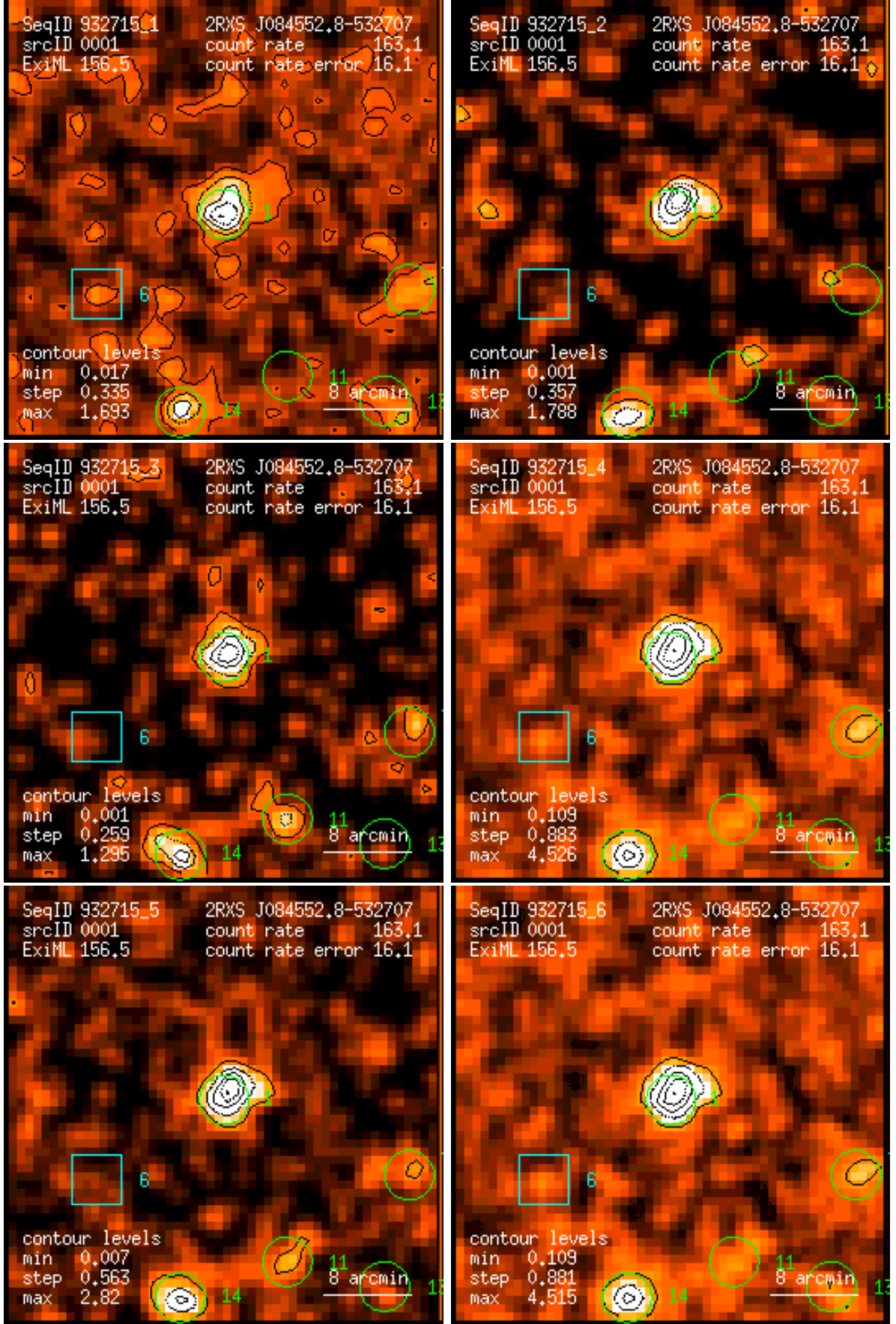
Figure 1: RASS 932715: detection 0001: band rate images, Gaussian filter: (1) PSPC channels 11 – 41, (2) 52 – 90, (3) 91 – 201, (4) 11 – 235, (5) 52 – 201, (6) 11 – 201. Broad band rates in counts/ks. Band rate contour levels in counts/ks/arcmin 2 .
