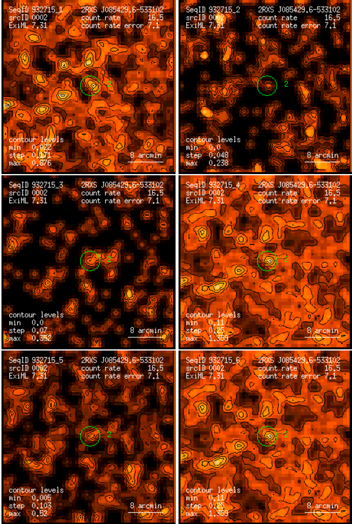
Figure 2: RASS 932715: detection 0002: band rate images, Gaussian filter: (1) PSPC channels 11 – 41, (2) 52 – 90, (3) 91 – 201, (4) 11 – 235, (5) 52 – 201, (6) 11 – 201. Broad band rates in counts/ks. Band rate contour levels in counts/ks/arcmin 2 .
