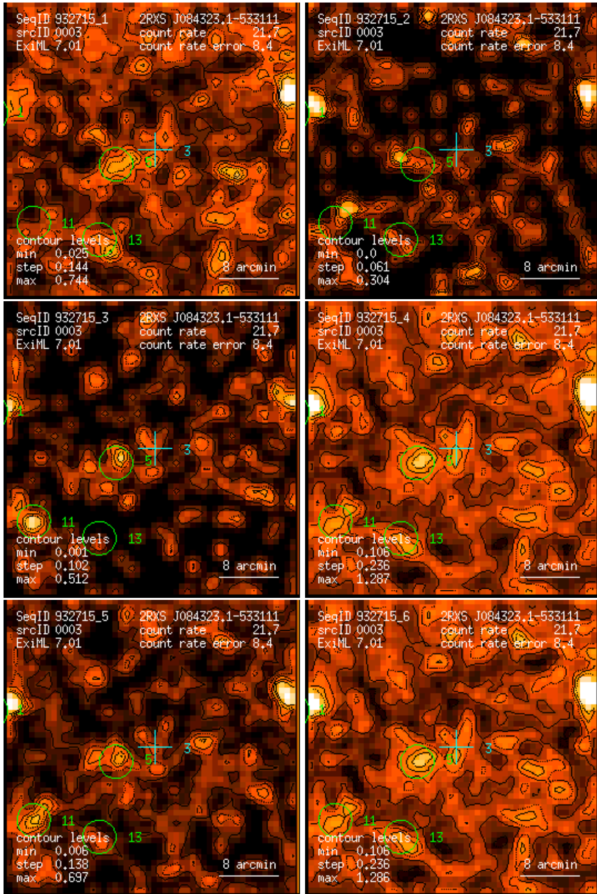
Figure 3: RASS 932715: detection 0003: band rate images, Gaussian filter: (1) PSPC channels 11 – 41, (2) 52 – 90, (3) 91 – 201, (4) 11 – 235, (5) 52 – 201, (6) 11 – 201. Broad band rates in counts/ks. Band rate contour levels in counts/ks/arcmin 2 .
