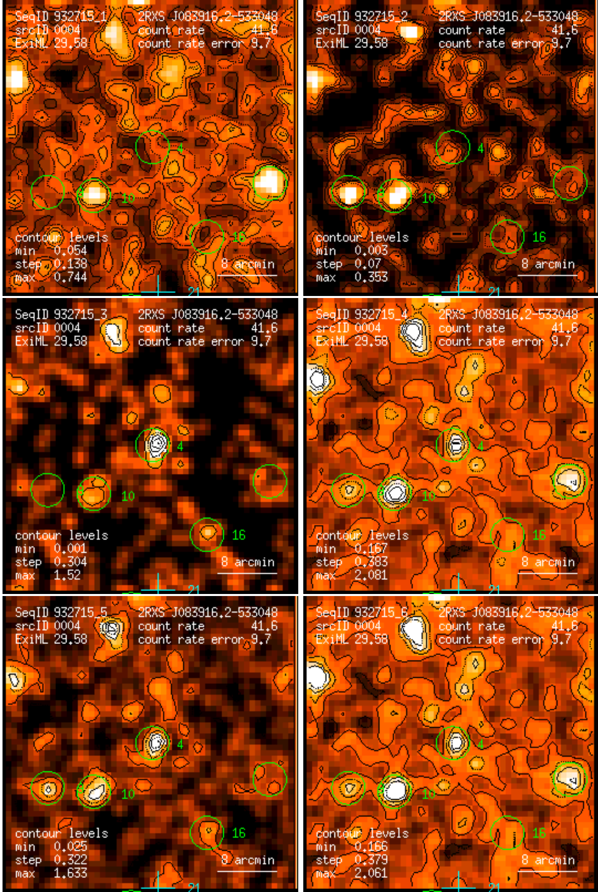
Figure 4: RASS 932715: detection 0004: band rate images, Gaussian filter: (1) PSPC channels 11 – 41, (2) 52 – 90, (3) 91 – 201, (4) 11 – 235, (5) 52 – 201, (6) 11 – 201. Broad band rates in counts/ks. Band rate contour levels in counts/ks/arcmin 2 .
