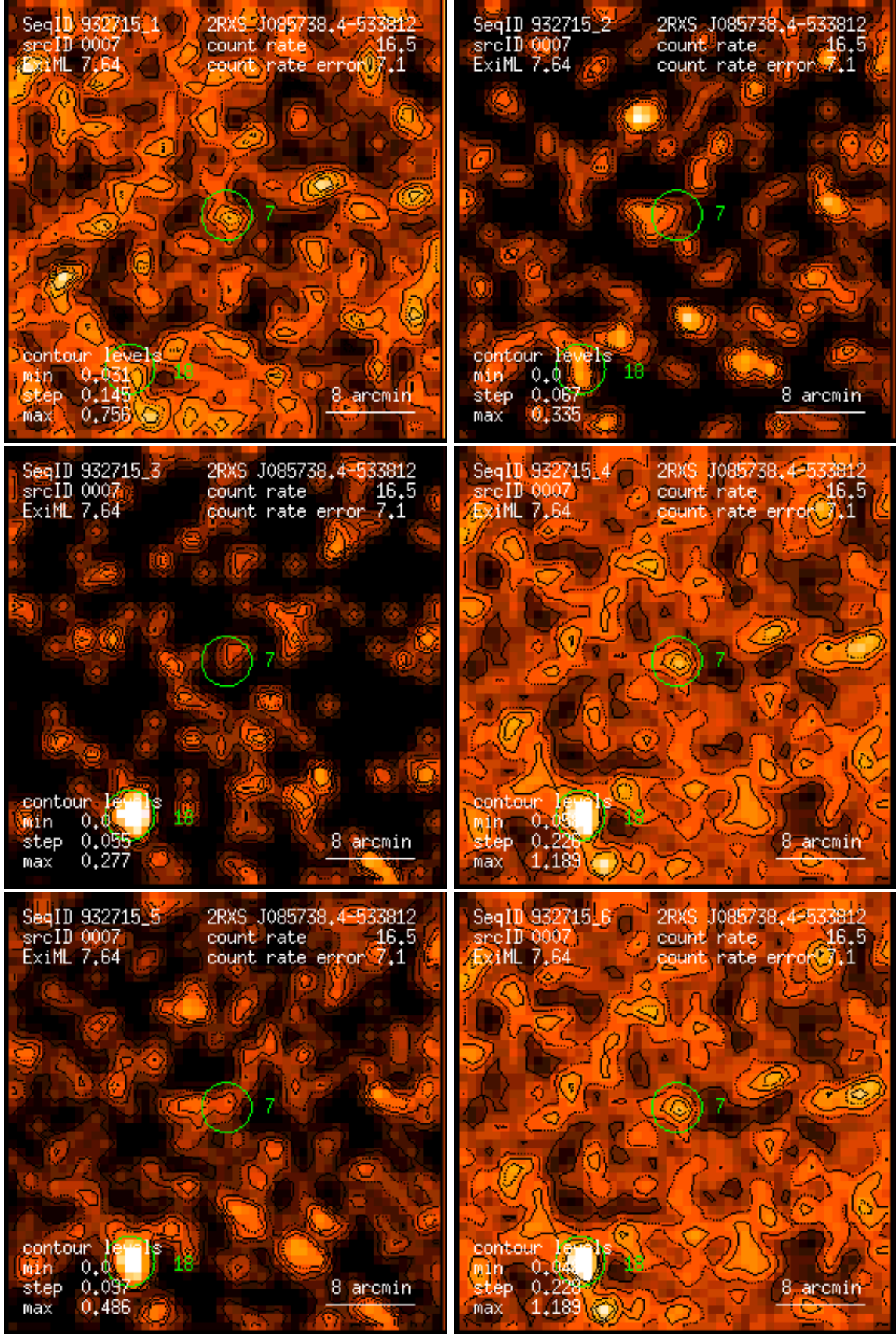
Figure 7: RASS 932715: detection 0007: band rate images, Gaussian filter: (1) PSPC channels 11 – 41, (2) 52 – 90, (3) 91 – 201, (4) 11 – 235, (5) 52 – 201, (6) 11 – 201. Broad band rates in counts/ks. Band rate contour levels in counts/ks/arcmin 2 .
