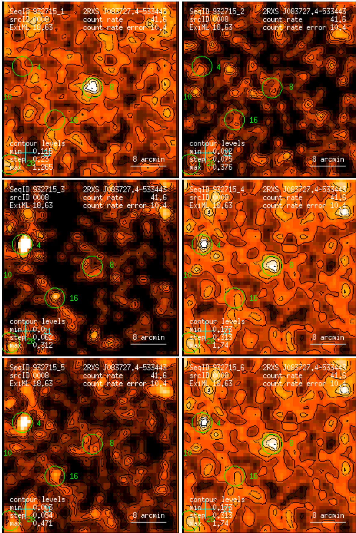
Figure 8: RASS 932715: detection 0008: band rate images, Gaussian filter: (1) PSPC channels 11 – 41, (2) 52 – 90, (3) 91 – 201, (4) 11 – 235, (5) 52 – 201, (6) 11 – 201. Broad band rates in counts/ks. Band rate contour levels in counts/ks/arcmin 2 .
