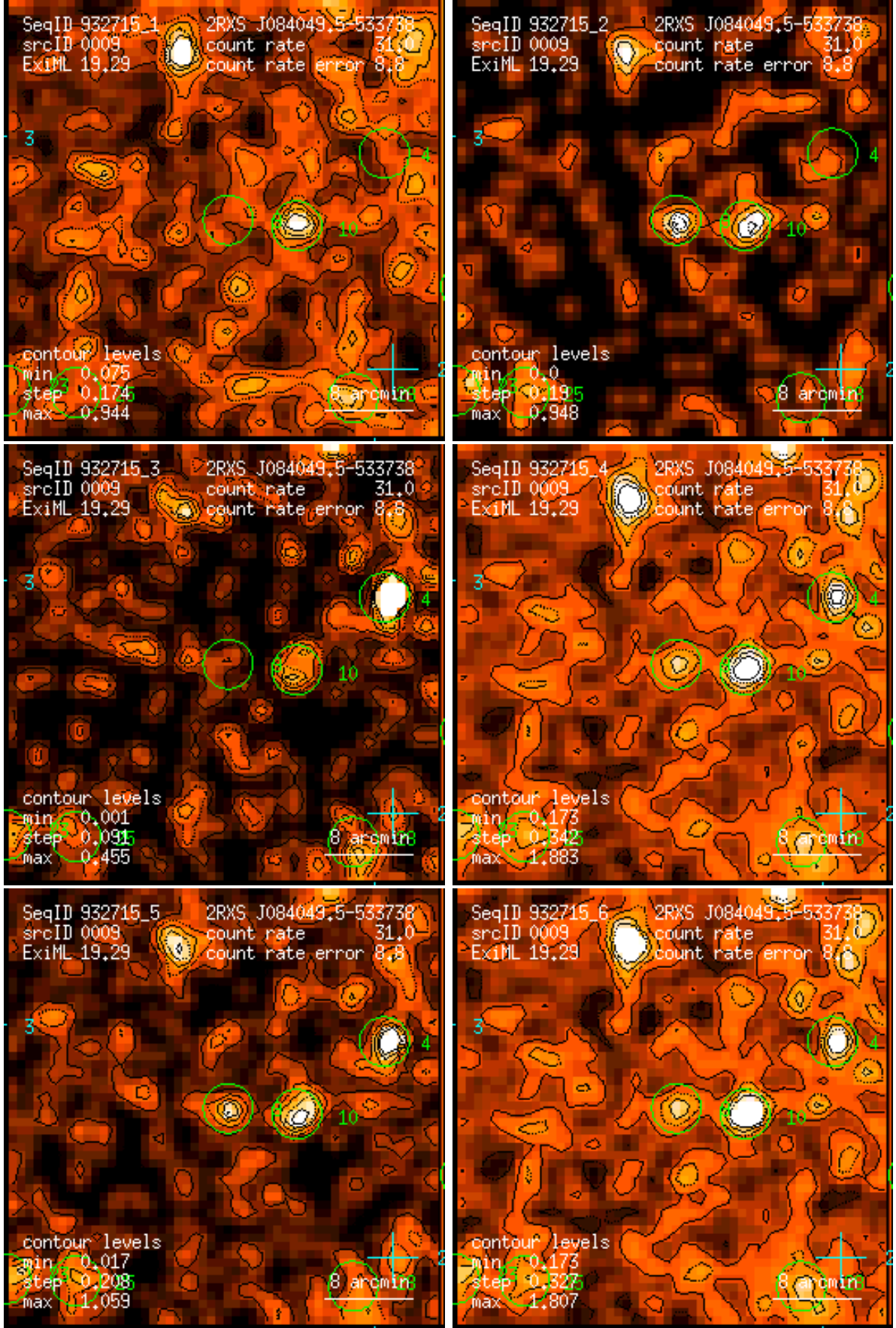
Figure 9: RASS 932715: detection 0009: band rate images, Gaussian filter: (1) PSPC channels 11 – 41, (2) 52 – 90, (3) 91 – 201, (4) 11 – 235, (5) 52 – 201, (6) 11 – 201. Broad band rates in counts/ks. Band rate contour levels in counts/ks/arcmin 2 .
