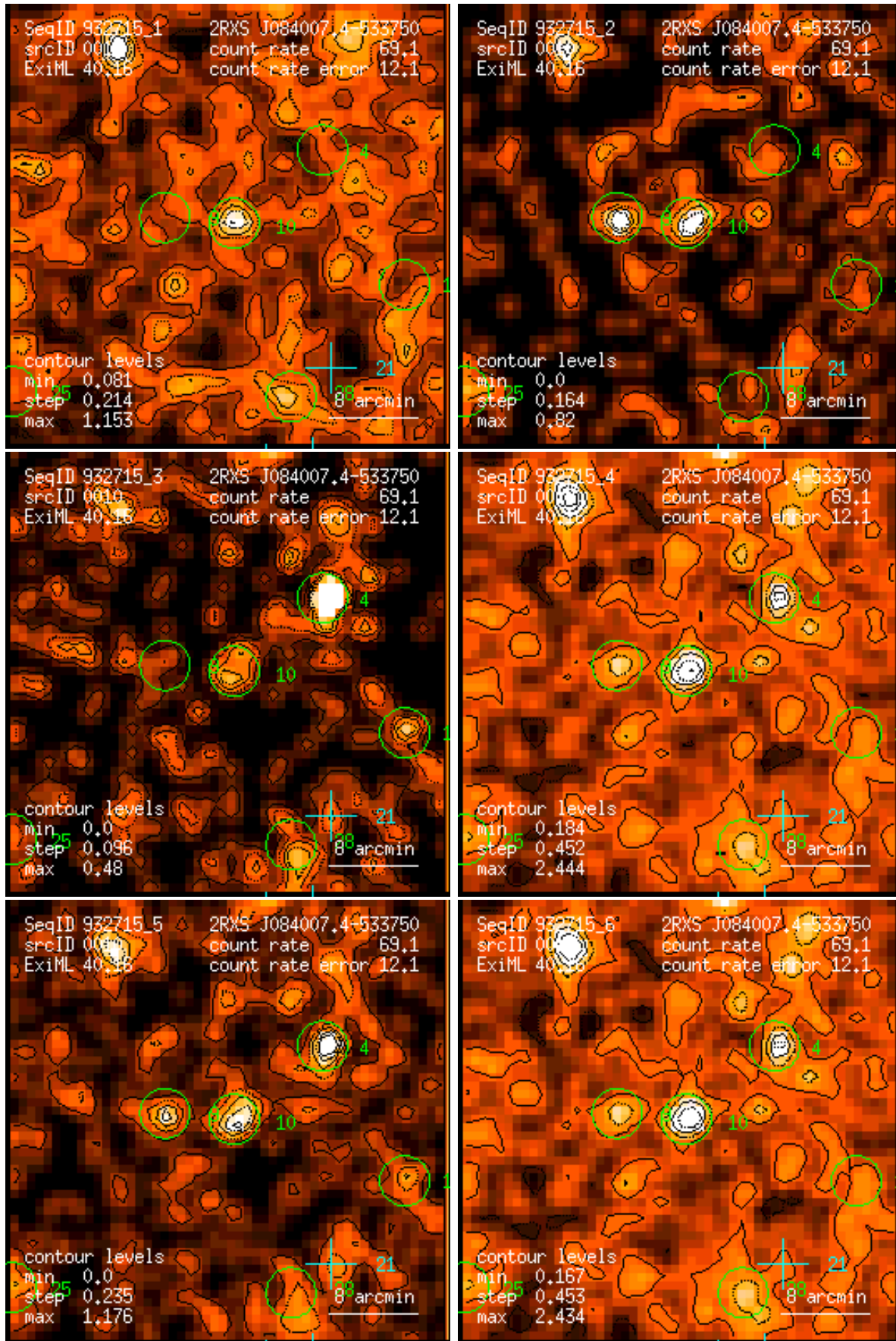
Figure 10: RASS 932715: detection 0010: band rate images, Gaussian filter: (1) PSPC channels 11 – 41, (2) 52 – 90, (3) 91 – 201, (4) 11 – 235, (5) 52 – 201, (6) 11 – 201. Broad band rates in counts/ks. Band rate contour levels in counts/ks/arcmin 2 .
