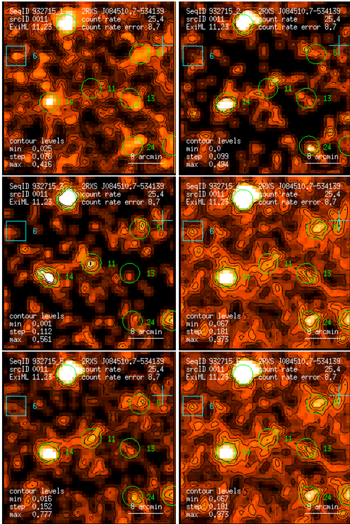
Figure 11: RASS 932715: detection 0011: band rate images, Gaussian filter: (1) PSPC channels 11 – 41, (2) 52 – 90, (3) 91 – 201, (4) 11 – 235, (5) 52 – 201, (6) 11 – 201. Broad band rates in counts/ks. Band rate contour levels in counts/ks/arcmin 2 .
